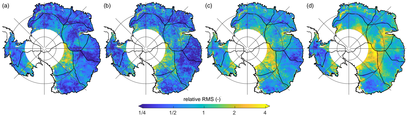
Figure 14. (a) Rms-RMS of (the time series of) the differences fv^{A1a} - fv^{A1b} . (b) Rms-RMS of the differences fv^{A1a} - fv^{A2a} . (c) Uncertainty estimate of fv^A : maximum rms-RMS of any combination of differences within versions of fv^A . (d) Rms-RMS of the residual differences r^{A1a} - r^{A2a} considering only the period after 2003. All rms-RMS maps (a–d) are normalised by the rms-RMS of fv^{Ma} .
