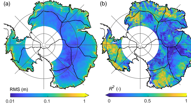
Figure 9. (a) Rms-RMS of the residual altimetric time series, r^{A1a} , for the period after 2003. (b) Values of R-squared for the regression A1a, R^2_{A1a} , considering the period after 2003. Colour bar arrows indicate that the value range exceeds the limits of the colour scale.
