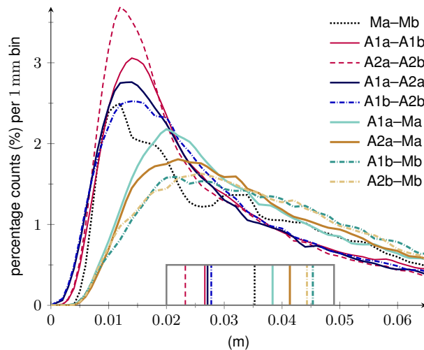
Figure 8. Histograms of the temporal \text{rmsRMS} , assessed at each grid cell, of differences between various versions of firn thickness variations. Vertical lines in the box indicate median values. Corresponding \text{rmsRMS} maps of differences are displayed in Fig. S15–S17.
