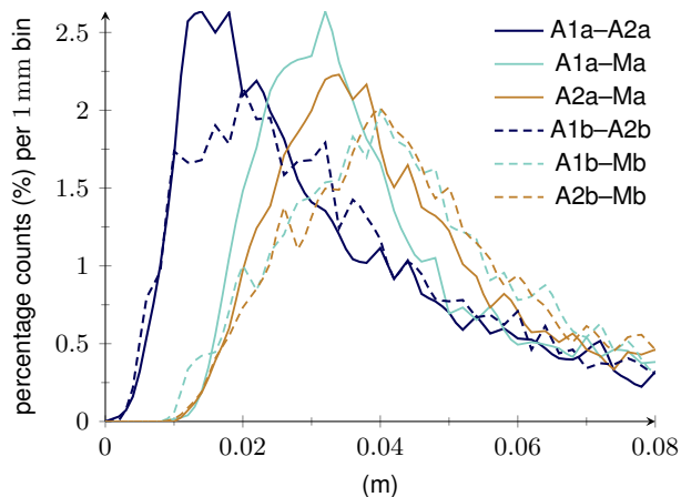
Figure 15. Histograms of the temporal rms RMS of differences between various versions of firn thickness variations assessed at each grid cell of basin 3.
