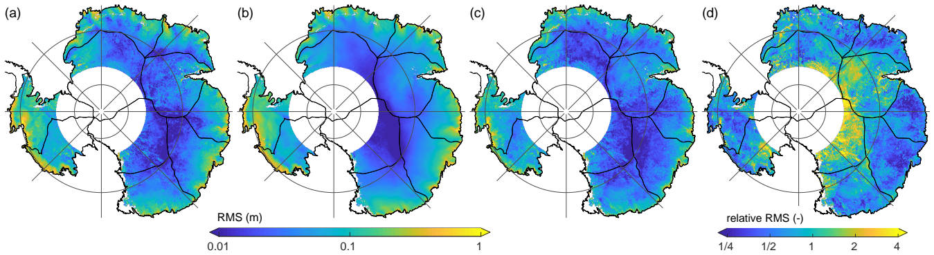
Figure 7. Root mean square ( \text{rmsRMS} ) of the times series of (a) adjusted firn thickness variations based on A1a, fv^{A1a} , and (b) modelled firn thickness variations based on Ma, fv^{Ma} . (c) \text{RmsRMS} of the time series of the differences fv^{A1a} - fv^{Ma} . (d) \text{RmsRMS} of the time series of the differences fv^{A1a} - fv^{Ma} divided by the \text{rmsRMS} of fv^{Ma} . All versions of fv^A and fv^M are illustrated in Fig. S15 and S16.
