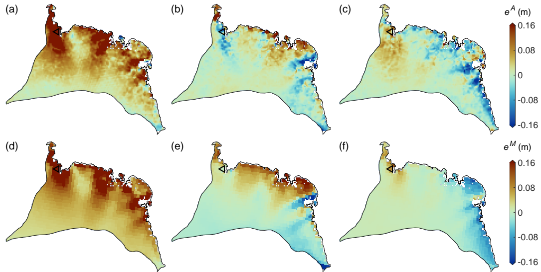
Figure 6. Scaling factors for basin 3. (a–c) e_{1...3}^{A1a} , first three observed factors from the regression A1a. (d–f) e_{1...3}^{Ma} , first three modelled factors from Ma. (d–f) is the same as Fig. 4a–c but with restored signal amplitudes for each grid cell. The location of P1 is shown by the black triangle.
