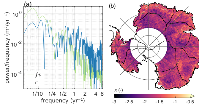
Figure 10. (a) Lomb-Scargle power spectral density ( psd-PSD ) of altimetric residuals, r^{A1a} , (blue) and adjusted firn thickness variations, fv^{A1a} , (green) for grid point P1. See Fig. S22 and S23 for the larger subset of selected grid points. (b) Spectral index \kappa for power-law noise adjusted to r^{A1a} of every grid cell. Colour bar arrows indicate that the value range exceeds the limits of the colour scale.
