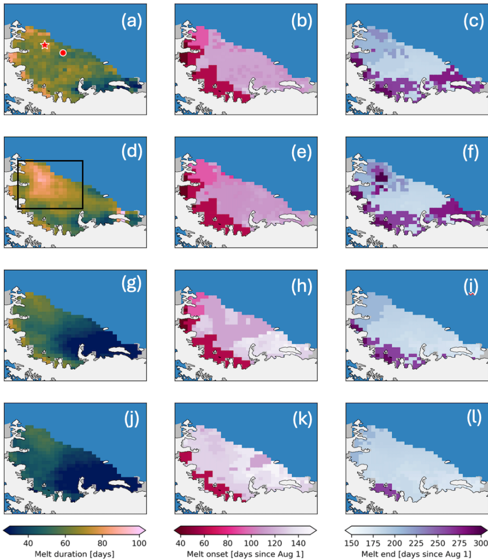
790 Figure 7: The Hybrid Method melt detection and three statistical thresholding techniques across the Larsen C. Red star and red circle in (a) is the location of AWS 14 and AWS 15, respectively. Black box in (d) represents area of high melt duration detected by Picard et al. (2023d). (a, d, g, j) represents melt duration for the 2013-2014 melt season (number of melt days) using the Hybrid Method, Picard et al. (2022), Torensini et al. (2003), and Zwally and Fiegles (1994), respectively. (b, e, h, k) represents melt onset in days since August 1 st 2013. (c, f, i, l) represents melt end in 795 days since August 1 st , 2013.
