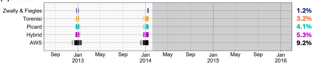
Figure 6: A comparison of melt detection between the Hybrid Method and three statistical thresholding techniques and AWS observations. Melt indicators from (a) AWS 17, (b) AWS 14, (c) AWS 15, (d) AWS 19, and (e) AWS 5. (a-e) Melt days when AWS surface energy balance melt > 0 (black lines). Melt days detected by Hybrid Method (purple
