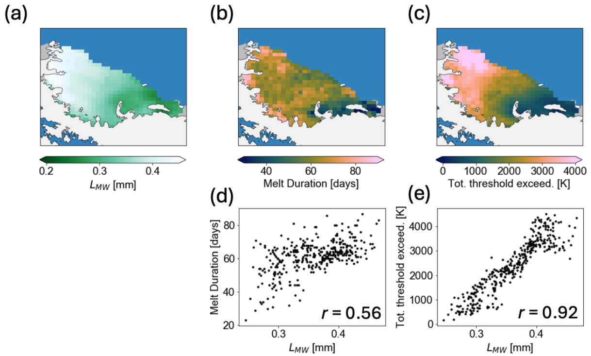
830 Figure 12: Larsen C (a) Microwave grain size ( L_{MW} ) from the Hybrid Method (March 2014 to end of June 2014). (b) Melt duration for the 2013-2014 melt season from the Hybrid Method. (c) Total threshold exceedance, or the integral between the Hybrid Method's dynamic threshold and AMSR-2 observations for the 2013-2014 melt season. (d) Scatter plot of melt duration and microwave grain size ( L_{MW} ). (e) Scatter plot of total threshold exceedance and microwave grain size ( L_{MW} ).
