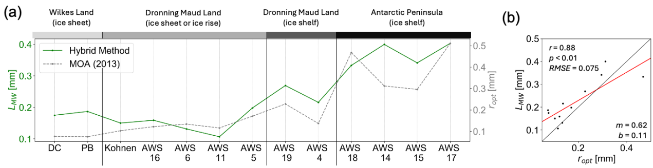
810 Figure 9: Comparison between microwave grain size from the Hybrid Method and optical grain radius from MODIS 2013 Mosaic of Antarctica (MOA). (a) Microwave grain size ( L_{MW} ; green line) and optical grain radius from MOA ( r_{opt} ; dashed grey line) from 13 AWS (Haran et al., 2018). (b) Scatter plot of microwave grain size ( L_{MW} ) and optical grain radius ( r_{opt} ). Data from both the Hybrid Method and Mosaic of Antarctica are from 2013-10-27 to 2013-12-16.
