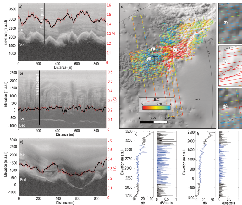
Fig. 2. Example radargrams from the AGAP North survey showing: (a) continuous englacial layers along RES survey line A44b, (b) discontinuous layering within RES survey line A29h and (c) absent layers in RES survey line A39d. In each panel, the continuity index (ILCI) is shown in red (unsmoothed), with a running mean of 10 traces highlighted by the black line. (d) Profile locations marked onto site-wide ILCI results (using a running mean of 100 traces). Background is BedMachine v2 bed topography (Mortlighem et al. , 2020). (e) A-scope plot demonstrating relative received power (dB) (left) and the absolute value of the gradient, for a trace in panel (a) (demonstrating continuous layering). (f) similar to (e), an A-scope of relative received power (left) and the absolute value of the gradient (right) for a trace in panel (b) (characterising disrupted layering). For both (e) and (f), the black line depicts the whole trace whilst the blue is the section used for calculation of the ILCI.
