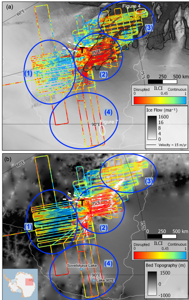
300 Fig. 3. ILCI analysis demonstrating the four zones of ILCI returns in the Lambert Glacier. White line is the Lambert-Amery catchment boundary (Zwally et al., 2012a) (a) ILCI smoothed over 100 traces, overlying MEASURE ice-surface velocity
