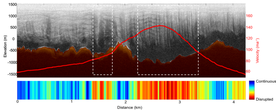
Fig. 4. Ice velocity (red curve) (Mouginot et al., 2019), bedrock traced from the radargram (brown shaded area), and Internal Layering Continuity Index (ILCI) returns from RES line A29C. White boxes highlight disrupted englacial layering where ice flows through the central rift and at the margin of Lambert Glacier. The location of this transect is noted in Fig. 3a. Birefringence patterns visible in the radargram, especially between 2 and 2.5 km and between 0-1000 m elevation, are discussed at the end of Section 4.1.
