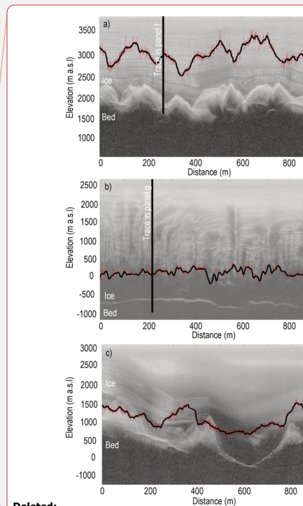
Fig. 2. Example radargrams from the AGAP North survey showing: (a) continuous englacial layers along RES survey line A44b, (b) discontinuous layering within RES survey line A29h and (c) absent layers in RES survey line A39d. In each panel, the continuity index (ILCI) is shown in red (unsmoothed), with a running mean of 10 traces highlighted by the black line. (d) Profile locations marked onto site-wide ILCI results (using a running mean of 100 traces). Background is BedMachine v2 bed topography (Mortlighem et al. , 2020). (e) A-scope plot demonstrating relative received power (dB) (left) and the absolute value of the gradient, for a trace in panel (a) (demonstrating continuous layering). (f) similar to (e), an A-scope of relative received power (left) and the absolute value of the gradient (right) for a trace in panel (b) (characterising disrupted layering). For both (e) and (f), the black line depicts the whole trace whilst the blue is the section used for calculation of the ILCI.
