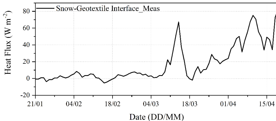
80 Figure S1. The top geotextile snow-interface heat flux at the Big Air Shougang.
