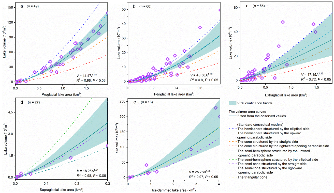
Figure 4. Relationships between the volume ( V ) and area ( A ) of glacial lakes were compiled in the present study for the following lake types: (a) proglacial lake, (b) periglacial lake, (c) extraglacial lake, (d) supraglacial lake, and (e) ice-dammed lake. The dotted lines indicate the volume curves of different standard conceptual models, which were fitted by Eq. (3).
