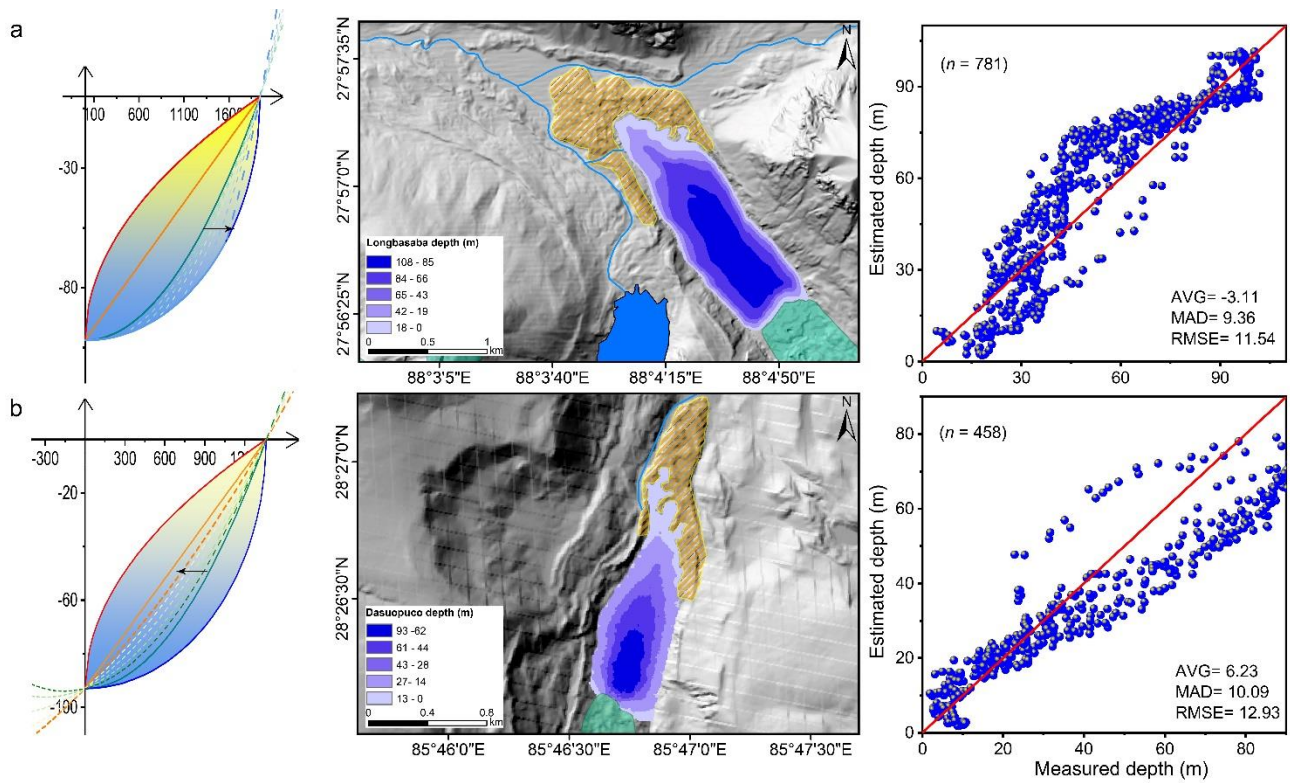
Figure 8. Modeled glacial lake bathymetric distributions of the two selected proglacial lakes. (a) Longbasaba Lake, and (b)Dasuopuco. The average deviation (AVG), mean absolute deviation (MAD), and root mean square error (RMSE) were selected to depict the consistency between the simulated and measured individual water depths along the boat routes. The movements of the general curves from one standard curve to another are also indicated.
