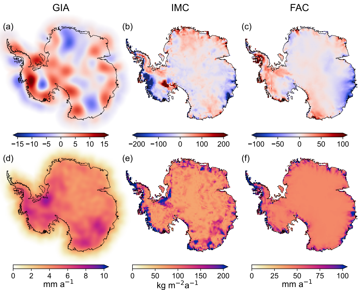
Figure 2: Maps of Antarctica illustrating the estimates of a) vertical bedrock motion due to glacial isostatic adjustment (GIA), b) surface density change due ice mass change (IMC) of the Antarctic Ice Sheet (AIS), and c) the thickness change of the firn air content (FAC) derived from the preferred inversion solution. (d-f) shows the 2\text{-}\sigma -uncertainties, respectively. Units indicated for (d-f) apply columnwise to (a-c).
