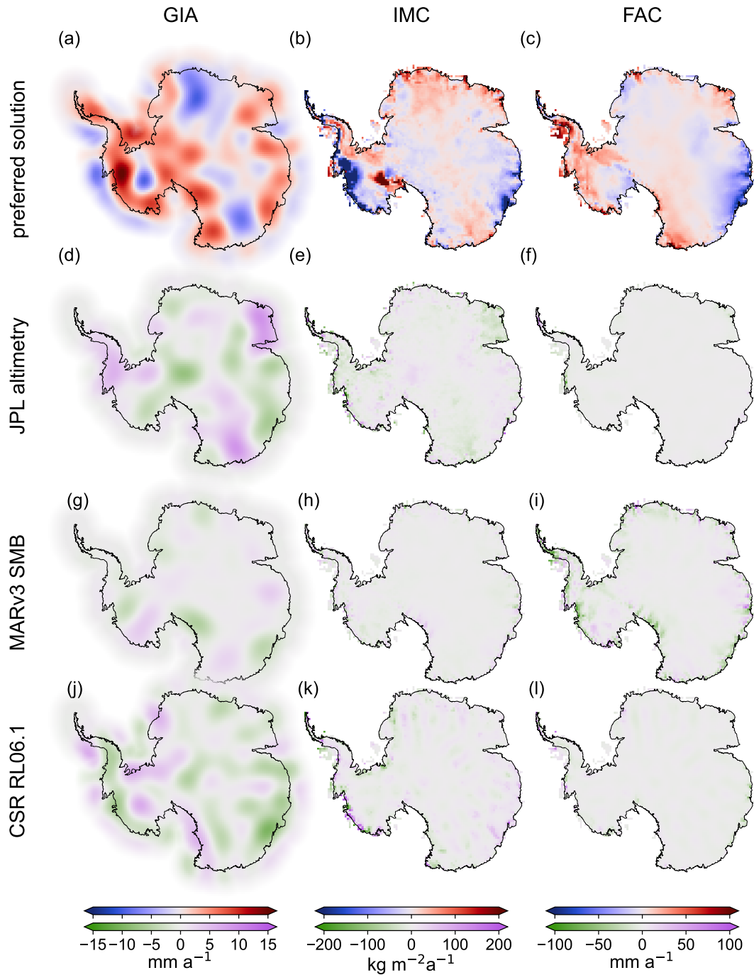
Figure 5: Assessment (3): Results from sensitivity tests using alternative input data sets (Fig. S9). The first row (a–c) shows the results from the preferred inversion result (Fig. 3). The second row (d–f) shows the differences between the inversion results and the first row where the surface elevation rate from (Nilsson et al., 2022, Fig. S9b) is used (test result minus preferred inversion solution). Similar, the third row (g–i) and fourth row (j–l) show differences to the inversion results with MARv3.11 SMB data (Kittel et al., 2021, Fig. S9c) and CSR RL06.1 gravitational fields (Pie et al., 2021, Fig. S9a), respectively.
