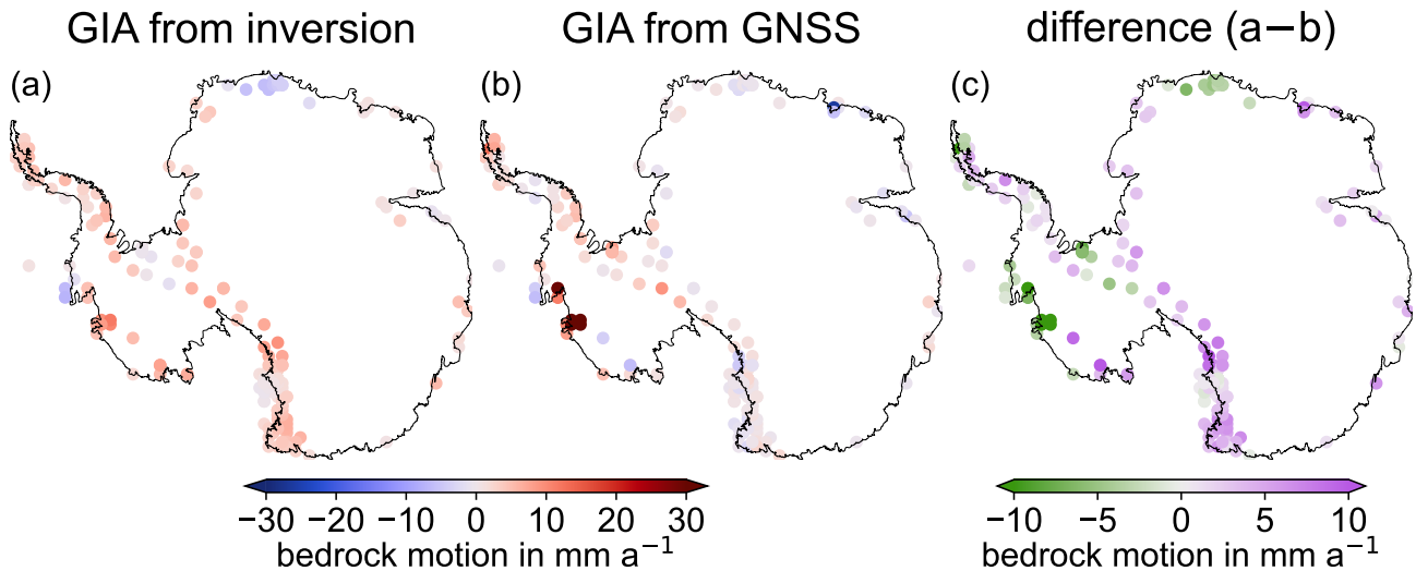
Figure 3: Assessment (1): Comparison of GIA-related bedrock motion at GNSS sites from the preferred inversion solution (a), from GNSS observations (b), and the difference between both (c).
