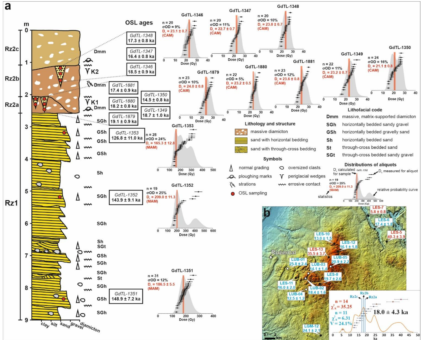
275 Figure 5: (a) Sediment profile of the entire exposed sequence with sedimentary features, OSL ages and distributions of equivalent doses measured for individual aliquots. (b) Spatial distribution of sampled boulders with ^{10}\text{Be} ages. New samples are indicated with white dots while recalculated samples are indicated with dark dots. Ages identified as outliers are marked in red, accepted ages are marked in blue. All ages are given in ka. Inset graph shows distribution of ^{10}\text{Be} ages with kernel density estimate curve and statistics before (red) and after (blue) excluding outliers. Bayesian ages of till layers Rz2a, Rz2b and Rz2c are also marked (blue lines) for comparison with ^{10}\text{Be} ages.
