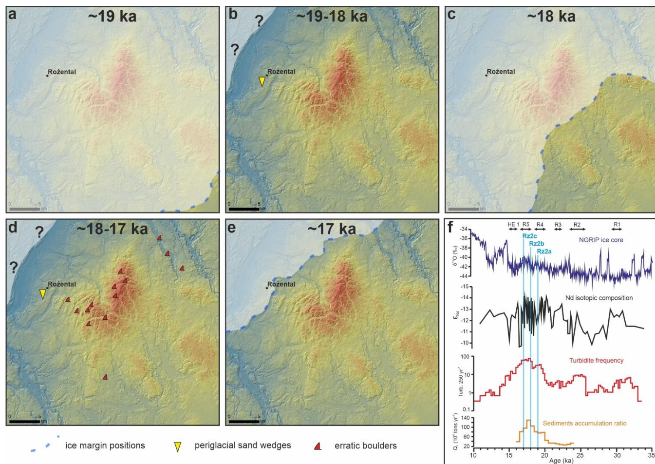
355 Figure 6: Reconstruction of palaeo-ice margin oscillations in the study area and millennial cycles recorded in marine sediments from the eastern edge of the North Atlantic with and in ice core record from Greenland. a) Maximum extent of the last FIS around 19 ka ago. (b) Ice-free conditions around 19-18 ka ago. (c) Ice sheet advance around 18 ka ago. (d) Ice-free conditions around 18-17 ka ago. (e) Ice sheet advance around 17 ka ago. (f) Variations of \delta^{18}\text{O} signature in NGRIP ice core (NGRIP-members, 2004), \epsilon_{\text{Nd}} isotopic composition, turbidite frequency and sediments load in marine sediments from the Bay of Biscay (for details see Toucanne et al., 2008, 2010 and 2015). Episodes of the Channel River large meltwater discharge (R-events) are marked as well as Heinrich event 1 (HE 1) and the most likely age of till ages for Rz2a, Rz2b and Rz2c.
