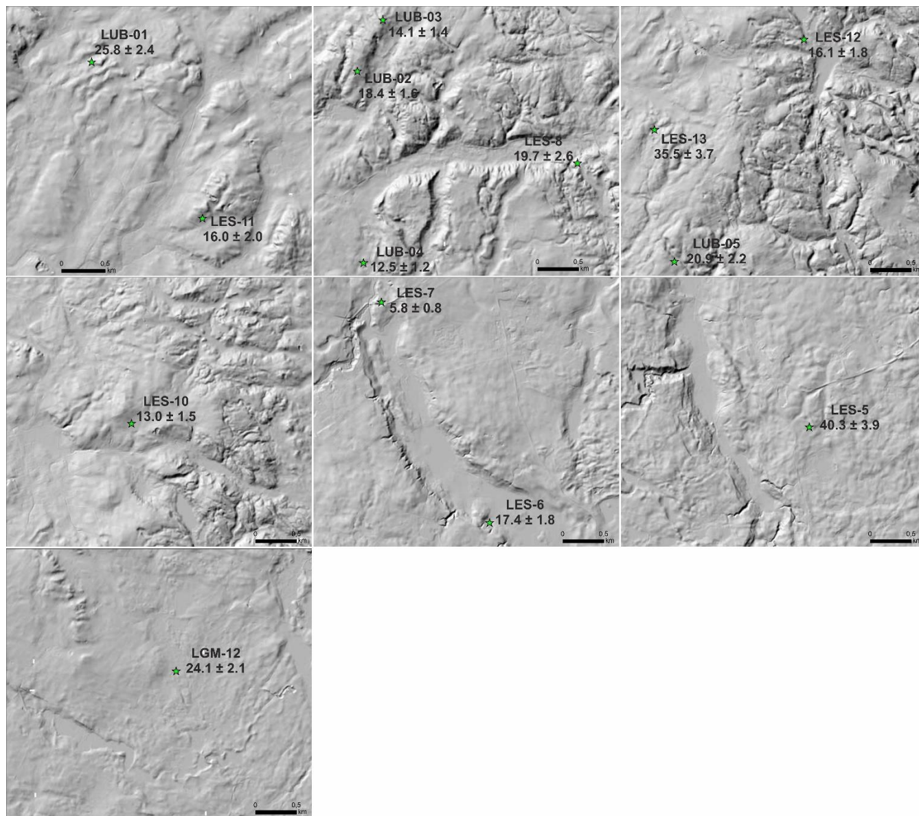
Figure A1: Location of erratic boulders used in this study against the high-resolution digital elevation model (LiDAR). Green stars indicate position of boulders, sample symbols and surface exposure ages (ka) are also given.
