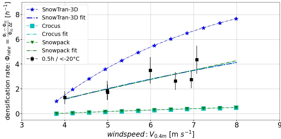
Figure 8. Densification rate as a function of wind speed for the Experiments 1-7 with constant air temperature ( T_a \approx -24 - 22^\circ\text{C} ) and experiment duration ( \tau_{exp} = 0.5 h) including the results of the SnowTran-3D (Liston et al., 2007) and the SNOWPACK (Lehning et al., 2002) and the CROCUS (Vionnet et al. 2012) model predictions and model fits to our experiments.
