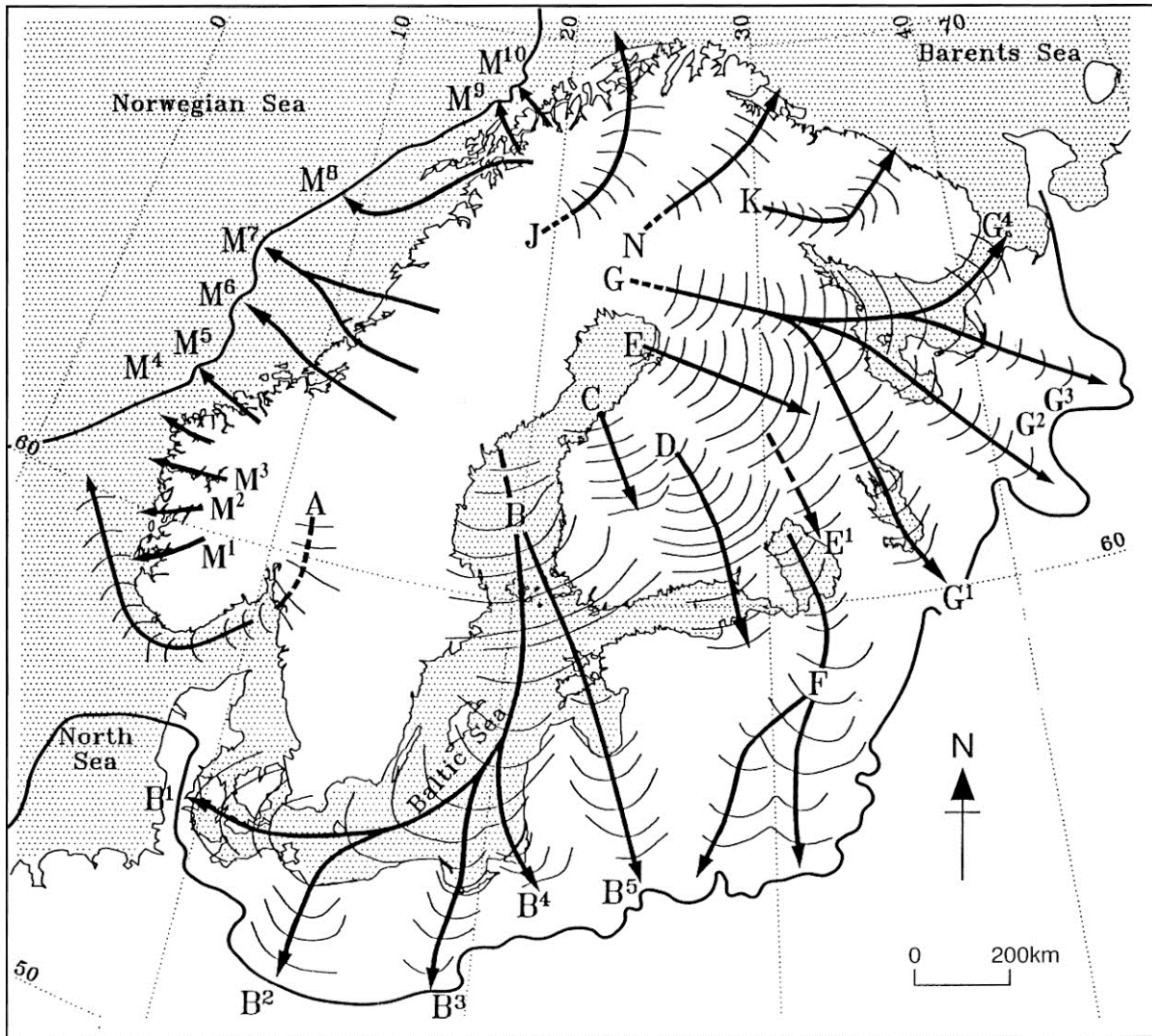
115 Figure 2. An early depiction of time-transgressive ice stream trajectories with associated back-stepping ice margins 120 after Boulton et al. (2001; Reprinted from Quaternary Science Reviews, 20/9, Boulton, G.S., Dongelmans P., Punkari, M., Broadgate, M., Palaeoglaciology of an ice sheet through a glacial cycle: the European ice sheet through the Weichselian, 591-625, Copyright (2001), with permission from Elsevier). The Baltic Sea depression is inferred to control the ice stream location but note that this depiction does not imply a synchronous Baltic Ice Stream of this length (>1000 km) branching into B1 to B4. Instead, it depicts numerous short length (<300 km) ice streams on land (B1 to B4) that, once back-stepped into the Baltic depression, eventually merged into a single ice stream. No submarine evidence was available at the time Boulton et al. (2001) drew the figure and it was the purpose of this paper to seek information about the footprint of this ice stream and its likely width. The relative timing of the ice streams draining the Baltic depression
