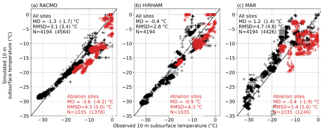
Figure 4. Evaluation of the monthly 10 m subsurface temperatures simulated by RACMO (a), HIRHAM (b) and MAR (c) against observations. The statistics presented are mean deviation (MD), root mean square difference (RMSD) and number of samples for which the comparison was possible (N) for the period when all three models are available (1980-2016). For RACMO and MAR, the statistics for all available measurements are given in the parenthesis. For sites where annual surface ablation is larger than snow accumulation, i.e., net ablation sites with a bare ice cover in summer, symbols and statistics are shown in red.
