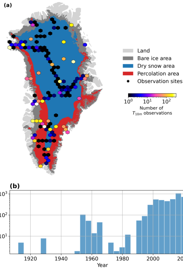
Figure 1. Spatial (a) and temporal (b) distribution of the T_{10m} observations in Greenland. Greenland surface classification according to Vandecrux et al. (2019) based on firn density profiles and remote sensing observations.
