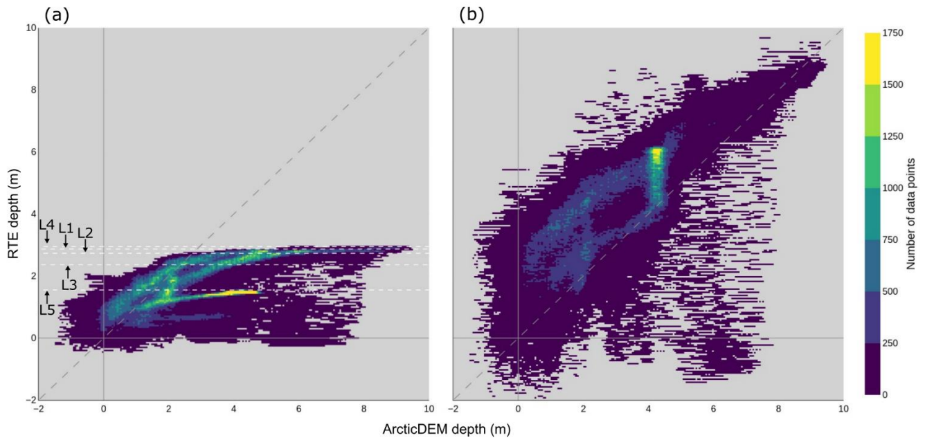
270 Figure 5: Density scatter plots of the depths derived from the red (a) and green (b) RTEs versus ArcticDEM depths for every pixel of the five lakes. The diagonal long-dashed lines represent one-to-one agreements between the depth datasets. The red-band RTE plateau depths are indicated by the labelled short-dash white lines in (a).
