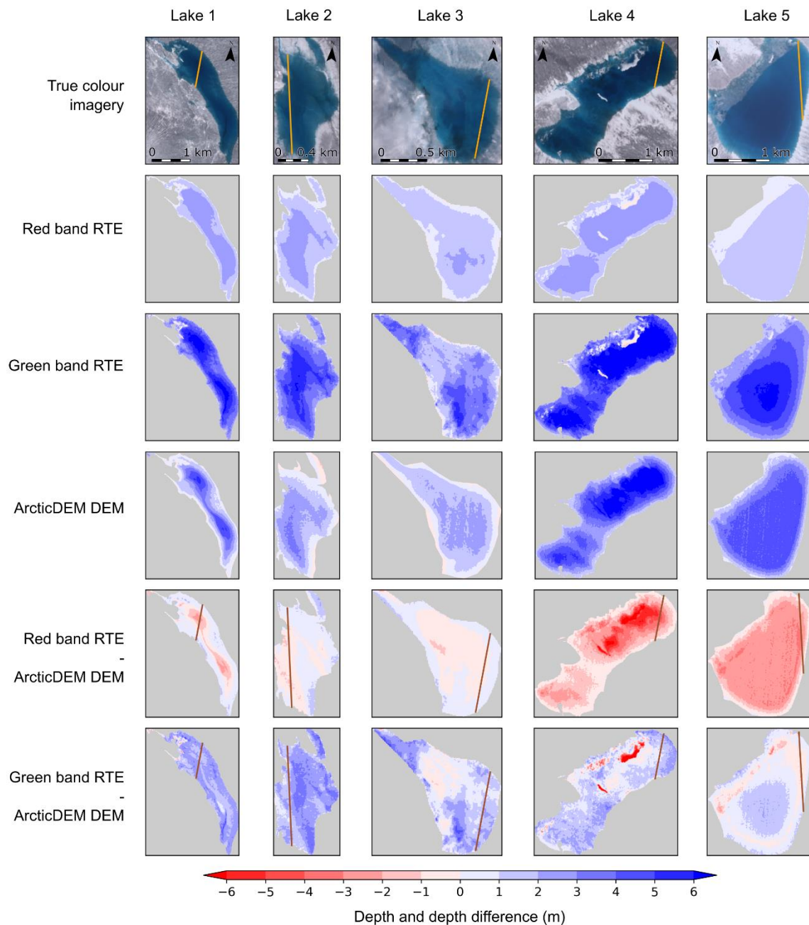
250 Figure 4: A comparison of red and green band RTE depths versus ArcticDEM depths in two dimensions. Each column shows results from one of our five study lakes, and each row shows information relating to a different retrieval method. The true colour imagery is from Sentinel-2 (Table A1). ICESat-2 transects are shown in orange on the true colour imagery and the depth difference plots.
