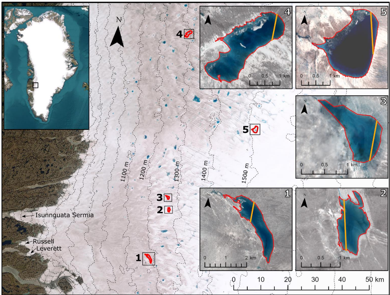
85 Figure 1: The locations of the five supraglacial lakes in relation to the study region. Contour lines calculated from the ArcticDEM 100 m mosaic are visible on the base map as grey dashed lines. The inset map indicates the location of the study area within Greenland. (1)–(5) show Lake 1 to Lake 5 in detail, where the background is a true colour image acquired on the date shown in Table A1 for each lake. The manually delineated lake outline is given in red, and the ICESat-2 transect is given in orange. The ICESat-2 ground tracks were cropped to the lake edges. The background images in panels (1)–(5) are the Sentinel-2 tiles detailed in Table A1. The base map data is courtesy of Earthstar Geographics via ESRI.
