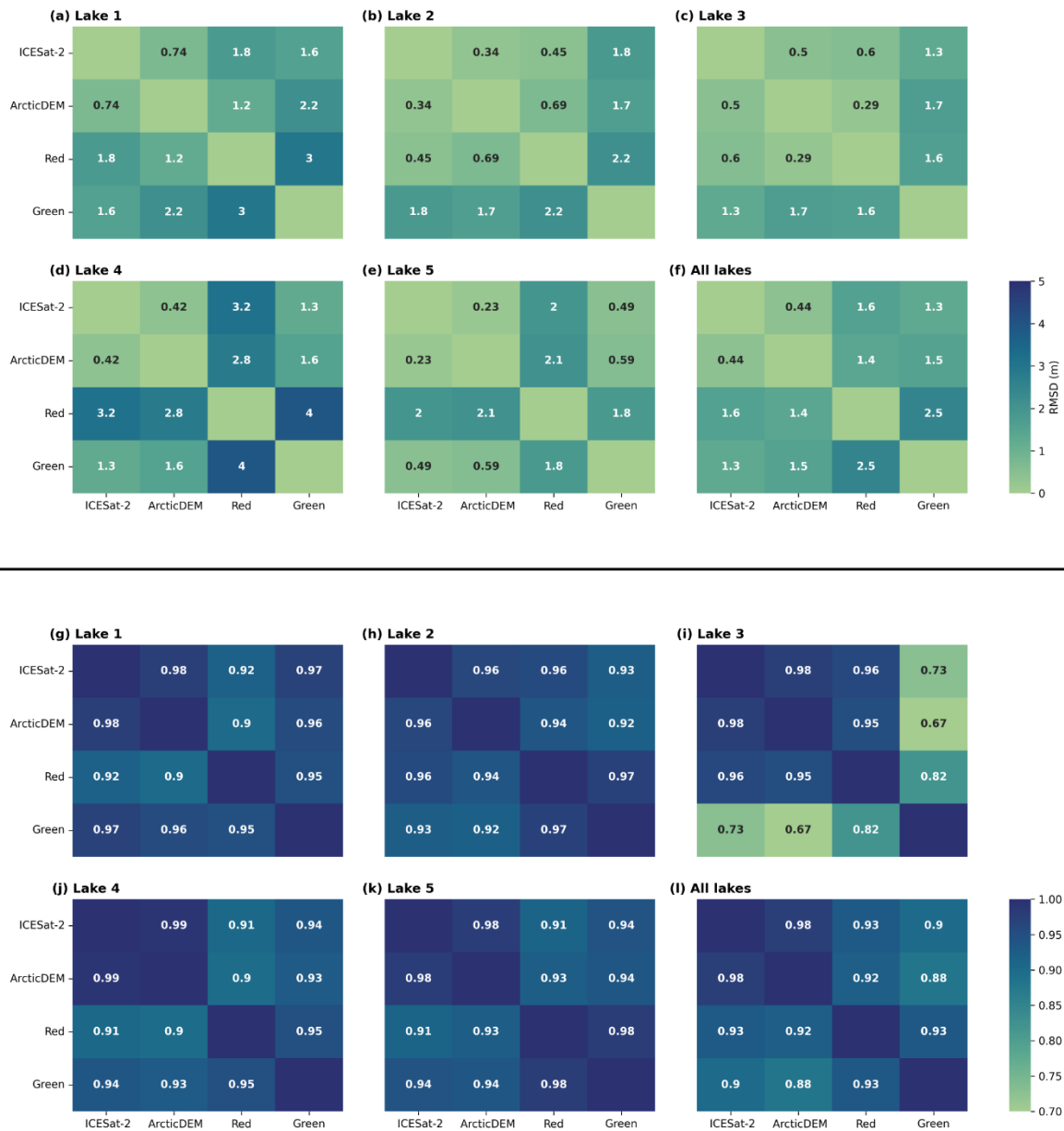
Figure 3: The root mean square difference (RMSD) and Pearson's correlation coefficients for each paired combination of depths derived from ICESat-2, ArcticDEM, red band RTE and green band RTE. (a)-(e) show the RMSD for Lake 1 to Lake 5, and (f) shows the average RMSD for all five lakes. (g)-(k) show the Pearson's correlation coefficient for Lake 1 to Lake 5, and (l) shows the average Pearson's correlation coefficient for all five lakes.
