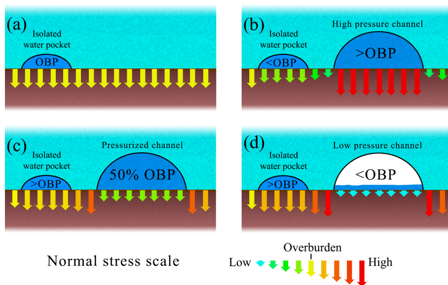
Figure 1. Effect of ice overburden and normal stress transfers on isolated water pockets. (a) In the absence of an active drainage system, the water pressure in an isolated water pocket reaches equilibrium close to overburden pressure. (b) A conduit with an internal water pressure above overburden reduces the normal stress in the surrounding bed leading to a pressure below overburden on nearby isolated water pockets. (c-d) A conduit with an internal water pressure below overburden increases the normal stress in the surrounding bed leading to above overburden pressures on isolated water pockets. Pressure variations in the channel would produce anti-correlated variations in the water pocket.
