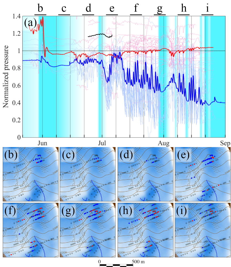
Figure 10. (a) Water pressure as a fraction of overburden for all correlated (blue) and anti-correlated (red) sensors participating in cluster H1. Thick lines represent mean values. The black line highlights a high-pressure correlated sensor, and the light blue shading the fraction of the glacier covered by fresh snow. Panels b to i show snapshots of the spatial distribution of correlated (blue circles) and anti-correlated (red circles) boreholes in eight time windows. Empty circles represent other boreholes that were recording pressure at the moment. The extent of the time windows associated with each snapshot is shown by the black bars at the top of panel a. The blue shading represents ice thickness.
