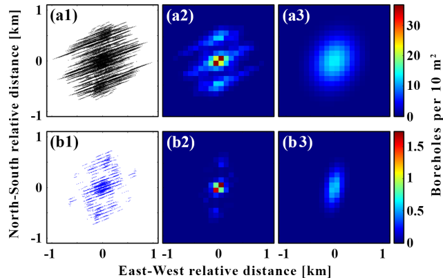
Figure 8. (a1) Relative positions of all 718,341 possible pairs of boreholes in selected time windows. (a2) Gridded density map of the relative positions in panel a1. (a3) Density map derived from the best bivariate Gaussian distribution fit to the relative positions in panel a1. (b1) Relative positions of all 9,514 pairs of boreholes identified as hydraulically connected in selected time windows. (b2) Gridded density map of the relative positions on panel b1. (b3) Density map derived from the best bivariate Gaussian distribution fit to the relative positions in panel a1.
