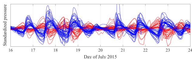
Figure 6. Diurnal residuals during 8 days for 50 sensors belonging to a hydraulic cluster. The two subclusters are presented in red and blue.
