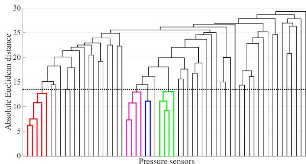
Figure 4. Example of a dendrogram computed by agglomerative hierarchical clustering over the 60 time series presented in panel a of Fig. 3. The coloured lines correspond to the four clusters shown in panels b–e of Fig. 3. The thick dotted line corresponds to a Split Point (SP) that would output the same four identified clusters. Diurnal residuals are normalized by their standard deviation, therefore, their values and their euclidean distances are dimensionless quantities.
