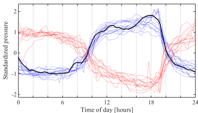
Figure 5. Best shapelet found for classification of mechanical connections (black line). This shapelet reached a 81% information gain (OSP = 12.9). For comparison, 23 time series of mechanical diurnal oscillations are also shown (blue and red lines).
