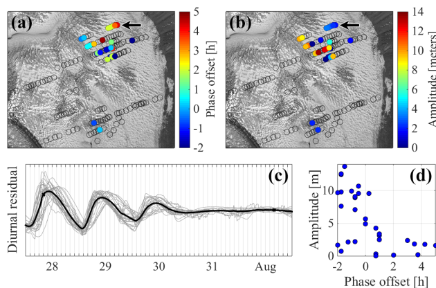
Figure 14. Spatial distribution of phase lag (a) and amplitude of diurnal variations (b), for the correlated boreholes in window g (July 27th to August 2nd, 2015) of cluster H1 (see Fig. 10). Panel c shows the individual diurnal residuals for each borehole as thin lines, and the mean diurnal residual for the cluster as a thick black line. Panel d shows the relationship between phase lag and amplitude.
