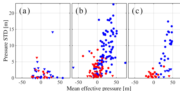
Figure 7. Scatter plots of mean effective pressure and pressure standard deviation for (a) mechanical cluster M1, (b) hydraulic cluster H1, and (c) window f of hydraulic cluster H1. Each point represents a borehole within the cluster. Boreholes that display diurnal variations in-phase with each other (i.e. belong to the same subcluster) are shown in the same colour. Boreholes are plotted as circles if located in the northern half of the study area or as triangles otherwise.
