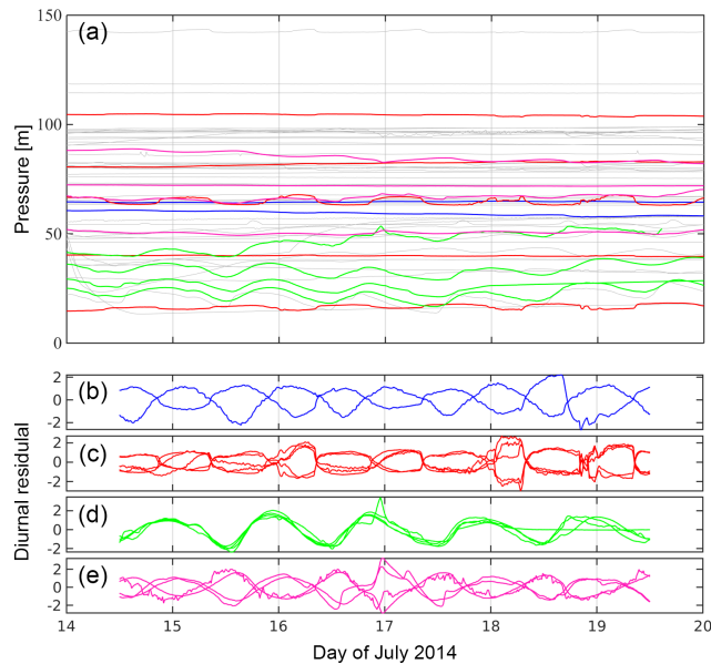
Figure 3. (a) Raw water pressure records of 60 time series over a 6-day window starting on July 14th, 2014. Time series belonging to four manually identified clusters are shown with thick lines. (b) to (e) Diurnal residuals of the sensors belonging to each of the four identified clusters (same colour coding of panel a). Diurnal residuals are normalized by their standard deviation, resulting in a dimensionless quantity.
