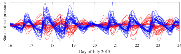
Figure 5. Diurnal residuals during 8 days for 50 sensors belonging to a hydraulic cluster. The two subclusters are presented in red and blue.
