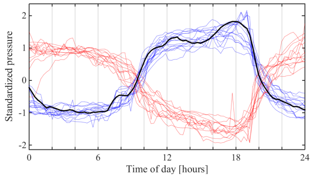
Figure 6. Best shapelet found for classification of mechanical connections (black line). This shapelet reached a 81% information gain (OSP = 12.9). For comparison, 23 time series of mechanical diurnal oscillations are also shown (blue and red lines).
