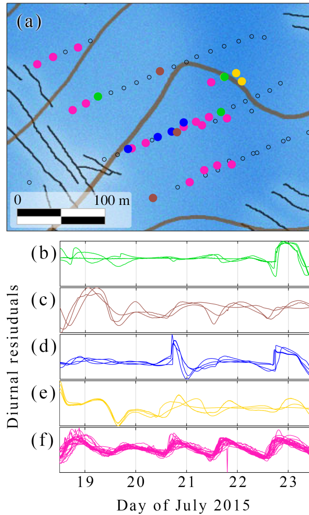
Figure 18. Detailed spatial distribution (a) and diurnal residuals (b-f) of five clusters observed in the plateau area between July 18th and 23rd, 2015. Only correlated boreholes are shown.
