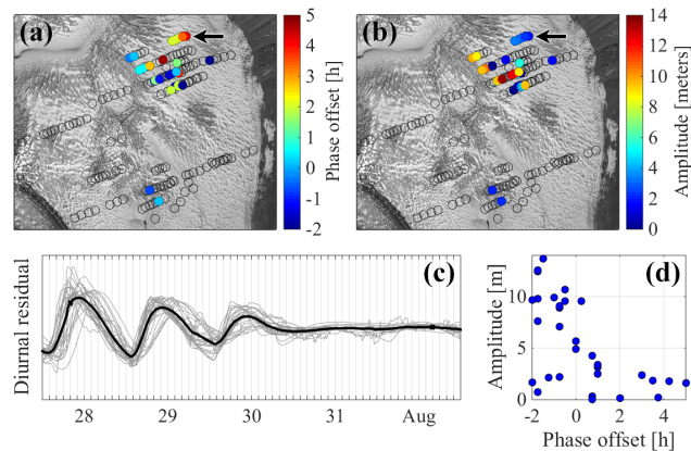
Figure 17. Spatial distribution of phase lag (a) and amplitude of diurnal variations (b), for the correlated boreholes in window g (July 27th to August 2nd, 2015) of cluster H1 (see Fig. 10). Panel c shows the individual diurnal residuals for each borehole as thin lines, and the mean diurnal residual for the cluster as a thick black line. Panel d shows the relationship between phase lag and amplitude.
