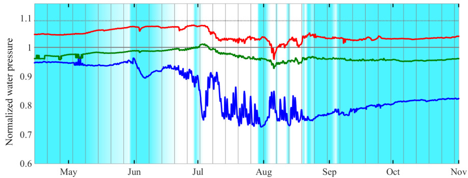
Figure 14. Glacier-wide spatially averaged mean water pressure values for three types of boreholes between May 15th and November 1st, 2015. In blue, the mean of 171 boreholes that at some point in the 2015 melt season were hydraulically connected. In green, the mean of 78 boreholes that participated in mechanical clusters but were never hydraulically connected. In red, the mean of 33 boreholes that were at some point anti-correlated members of a hydraulic cluster but were never hydraulically connected. All water pressure values used to compute these means were normalized by the overburden pressure of each corresponding borehole. Light blue shading represents the approximate surface snow cover using the same color scale as Fig. 10.
