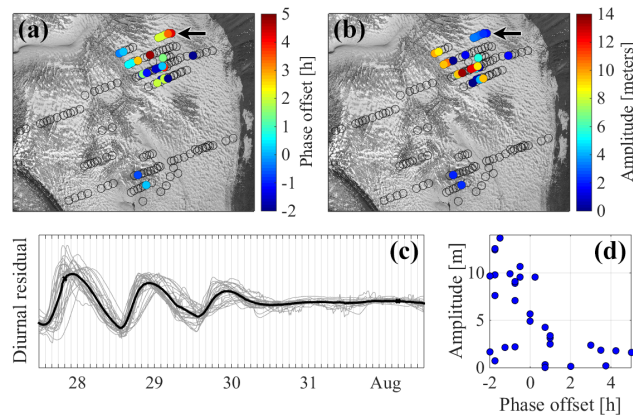
Figure 17. Spatial distribution of phase lag (a) and amplitude of diurnal variations (b), for the correlated boreholes in window g (July 27th to August 2nd, 2015) of cluster H1 (see Fig. 10). Panel c shows the individual diurnal residuals for each borehole as thin lines, and the mean diurnal residual for the cluster as a thick black line. Panel d shows the relationship between phase lag and amplitude.
