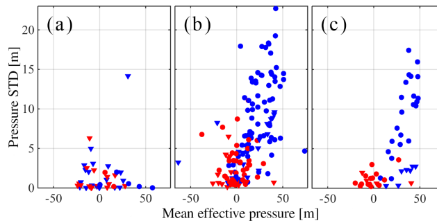
Figure 7. Scatter plots of mean effective pressure and water pressure standard deviation for (a) mechanical cluster M1, (b) hydraulic cluster H1, and (c) a six-day window f-of-on hydraulic cluster H1: this time window corresponds to window f defined on Figs. Each- 10 and 11. In all panels, each point represents a borehole within the cluster. Boreholes that display diurnal variations in-phase with each other (i.e. belong to the same subcluster) are shown in the same colour. Boreholes are plotted as circles if located in the northern half of the study area or as triangles otherwise.
