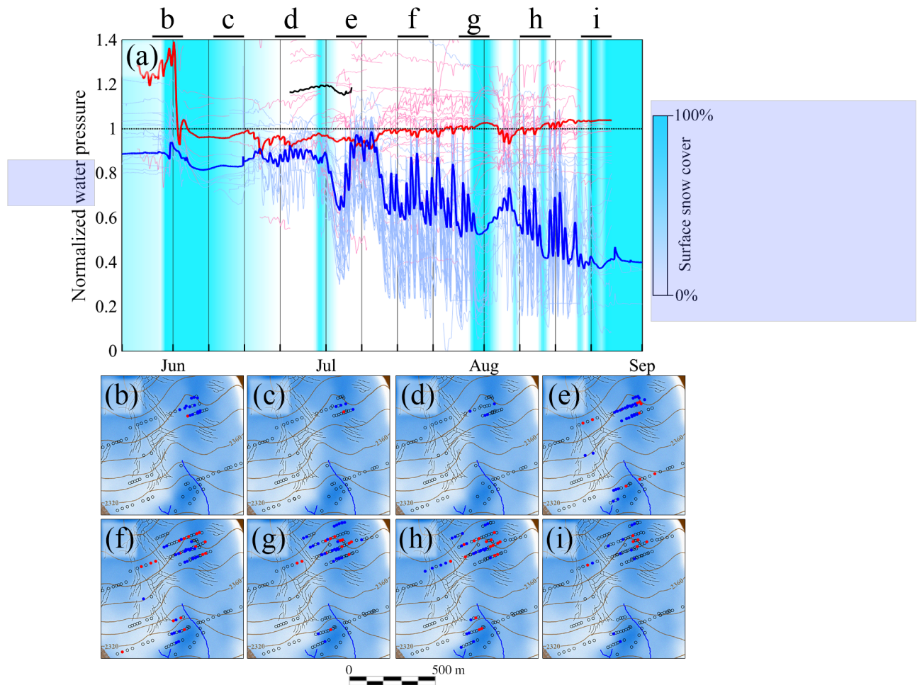
Figure 10. (a) Water pressure as a fraction of overburden for all correlated (blue) and anti-correlated (red) sensors participating in cluster H1. Thick lines represent mean values. The black line highlights a high-pressure correlated sensor, and the light blue shading the fraction of the glacier covered by fresh snow. Panels b to i show snapshots of the spatial distribution of correlated (blue circles) and anti-correlated (red circles) boreholes in eight time windows. Empty circles represent other boreholes that were recording water pressure at the moment. The extent of the time windows associated with each snapshot is shown by the black bars at the top of panel a. The blue shading represents ice thickness.
