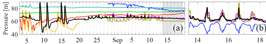
Figure 13. (a) Water pressure in a hydraulic cluster observed in August 2015 that we then identified as a mechanical in mid-September 2015. (b) Diurnal residual for the period between September 14th and 18th 2015, using the same colour coding of panel a. It can be seen how the sensor in black transitioned from displaying a large amplitude hydraulic signal to small amplitude one, characteristic of mechanical clusters.
