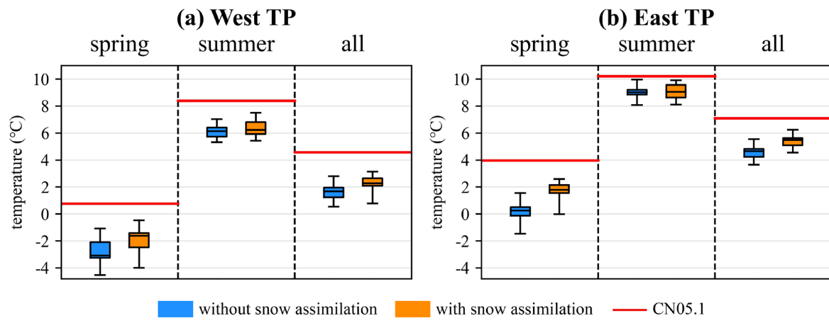
Figure S1. The daily averaged temperature of the two ensemble reforecasts and CN05.1 data in the (a) west Tibetan Plateau and (b) east Tibetan Plateau.
