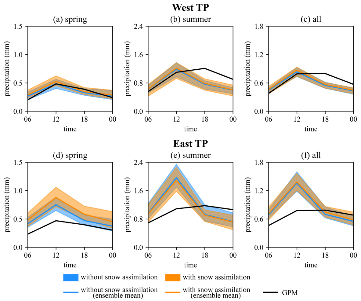
Figure S4. The precipitation diurnal cycles for the two ensemble reforecasts and GPM data.
