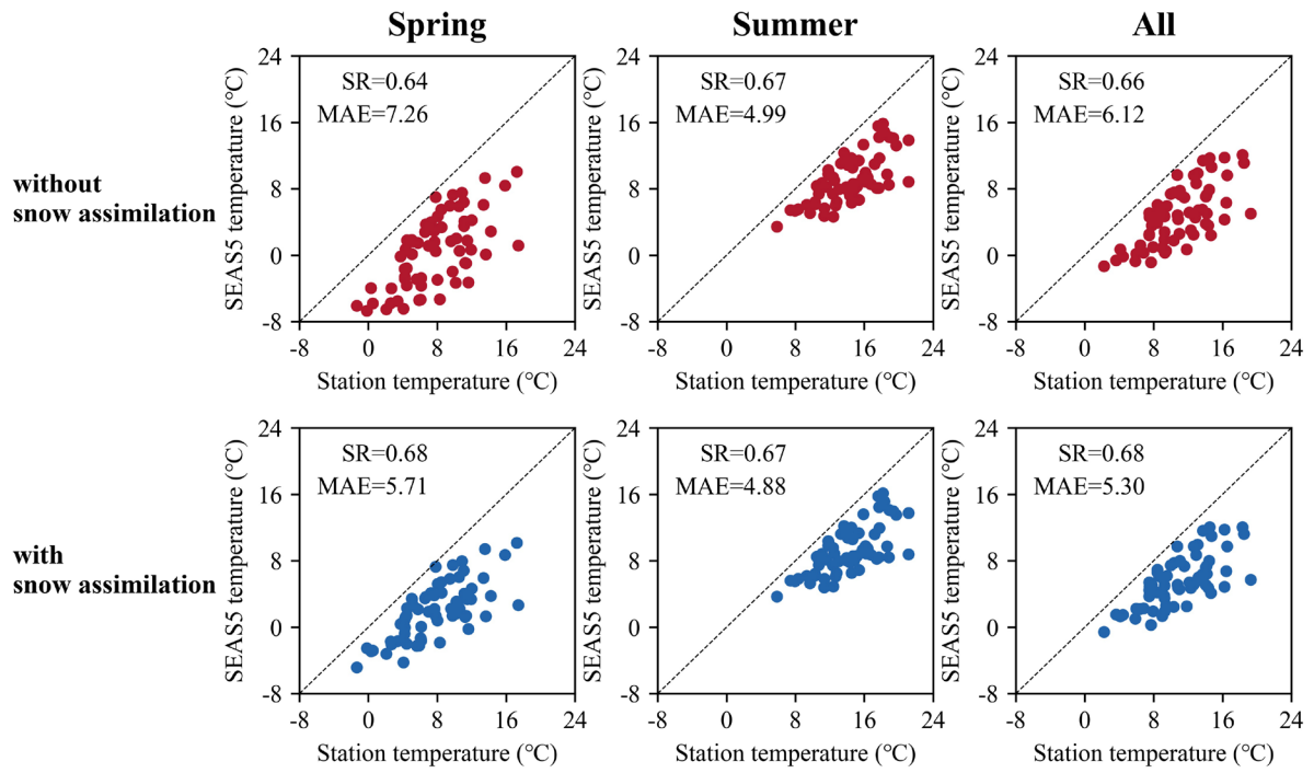
Figure S2. The spatial correlations and mean error between the temperature reforecasts and in-situ observations.
