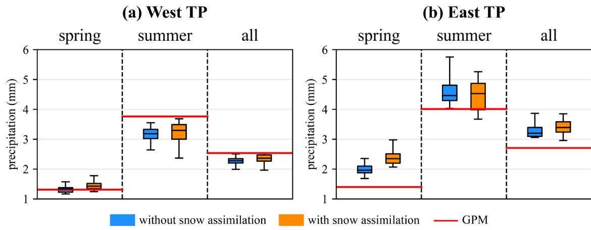
Figure S3. The daily averaged precipitation of the two ensemble reforecasts and GPM data in the (a) west Tibetan Plateau and (b) east Tibetan Plateau.
