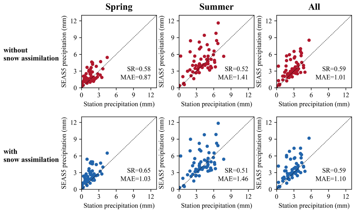
Figure S5. The spatial correlations and mean error between the precipitation reforecasts and in-situ observations.
