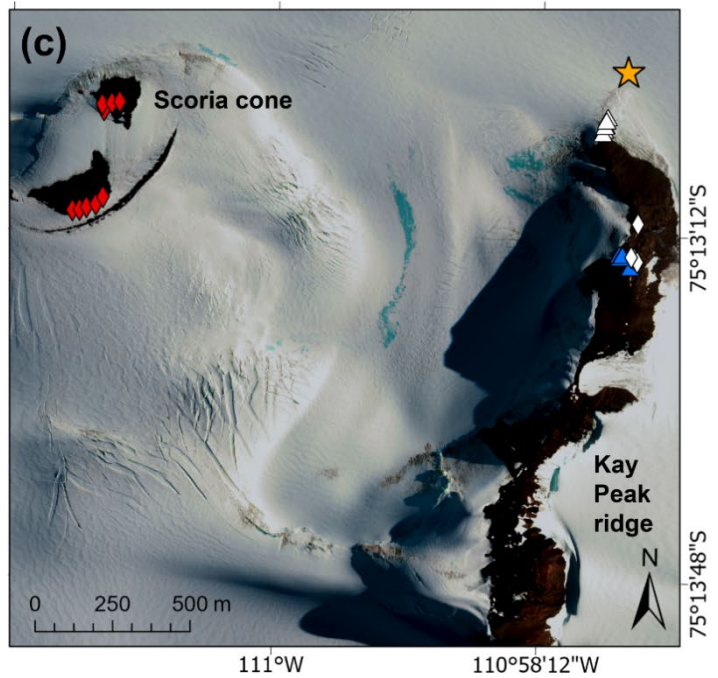
Figure 1: Location of the study area in the context of Mt Murphy and the wider ASE. (a) ASE area map displaying regional ice streams, ice velocities (Mouginot et al., 2012) overlaid on Reference Elevation Model of Antarctica (REMA) (Howat et al., 2019) regional bathymetry (Arndt et al., 2013), 2011 grounding line (black line; Rignot et al., 2011) and Antarctic coastline (blue; Antarctic Digital database, version 7.2). (b) Mt Murphy site map generated using REMA derived hill shade, with contours representing 100 m intervals. Locations of previous exposure ages (Johnson et al., 2020, 2008) indicated by coloured symbols shown in Fig. 1b key, also displayed are both the 2011 grounding line (same as in Fig. 1a), and most recent localised grounding line (red dotted; Milillo et al., 2022). (c) High resolution satellite imagery (732 false colour composite), DigitalGlobe Products, WorldView 2 © 2013 DigitalGlobe, Inc., a Maxar company showing scoria cone and Kay Peak Ridge. Drill site indicates subglacial bedrock core recovery by the Geological History Constraints (GHC) subglacial drilling project (Boeckmann et al., 2021).
