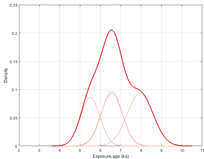
Figure A2: Kernel density estimate plot of ^{14}\text{C} ages distribution for lower Kay Peak Ridge ( n=4 ), with the two youngest ages (KAY 105, KAY 109) removed. Error weighted mean: 6472; Standard error: 266; External error: 205; reduced chi-squared: 3.29; chi-squared p-value: 0.0196
