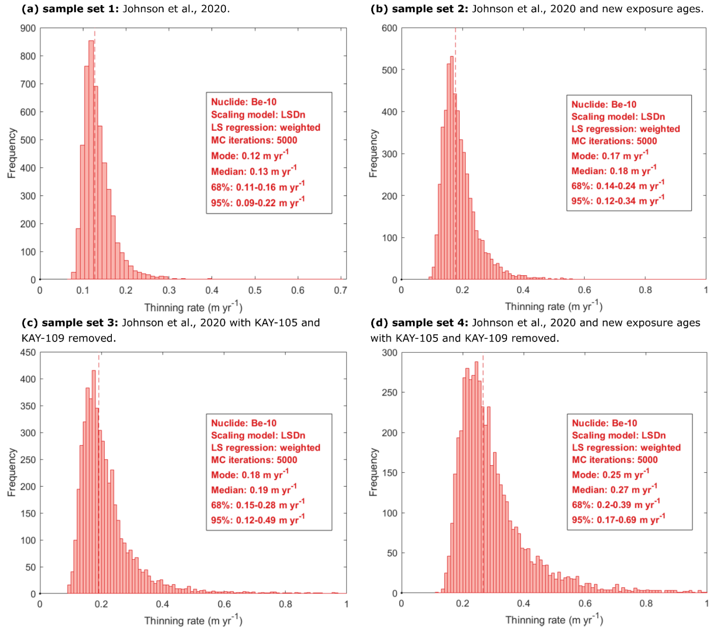
Figure B1: Histogram outputs of ice surface thinning rates generated by iceTEA (Jones et al., 2019). Results of linear regression: (a) the original sample set of Johnson et al. (2020), (b) incorporating new data from Scoria Cone, (c) removing young ages identified as outliers and (d) incorporating new data from Scoria Cone as well as removing young ages identified as outliers. Panel boxes inset in each subfigure display the median and modal values for thinning rates as well as the range of 68 % and 95 % confidence intervals.
