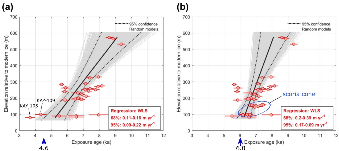
Figure 6: Linear regression transects of ice surface lowering over time (ka) relative to the modern ice surface (m). (a) Results of linear regression using the same exposure ages as Johnson et al. (2020). (b) Results of linear regression using new scoria cone ^{10}\text{Be} exposure ages with KAY-105 and KAY-109 outliers removed. In both panels, exposure ages are plotted relative to elevation above the modern ice surface and display ( 1\sigma ) external errors. Modern ice surface elevations are as reported in Johnson et al., 2020, and using 80 m asl as the modern ice surface elevation adjacent to the scoria cone site. The dotted black lines delimit the 95% confidence intervals of the thinning profile (also shown in Fig. 5b). The straight black line displays the model best fit line and grey lines represent all model fits to the data. Surface exposure age elevations were input normalised to the height above the modern ice surface at Kay Peak (80 m). The blue arrows indicate timing ice surface reached its current elevation based on extrapolation of the best fit line for each transect. The blue ellipse in panel b indicates the position of scoria cone exposure ages on the linear regression transect. See Fig. A4 for the linear regression transects generated from Sample Sets 2 and 3.
