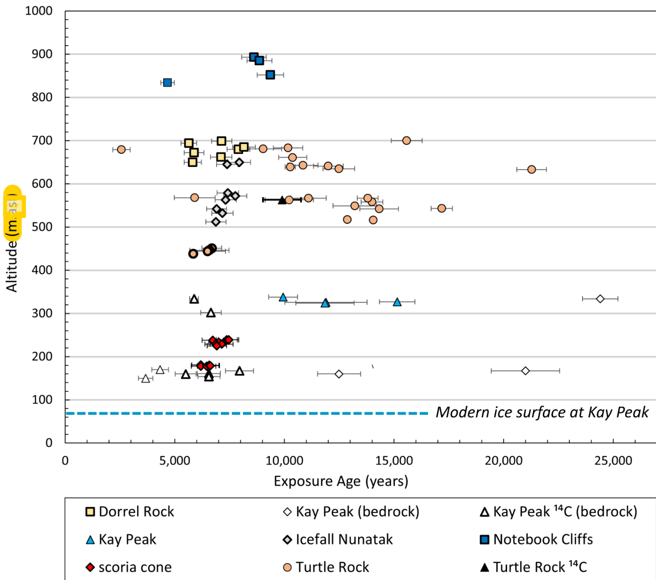
320 Figure 7: New exposure ages obtained from scoria cone in comparison with exposure age data reported by Johnson et al. (2008; 2020) for nunataks surrounding Mt Murphy. Exposure ages are plotted as 10 Be and in situ 14 C exposure ages (years) versus altitude (m asl). Filled symbols represent erratics and open symbols represent bedrock samples, all symbols represent 10 Be exposure ages unless specified as in situ 14 C in the key. Bold outline indicates samples used for Sample Set 4 linear regression analysis. Dashed blue lines show the modern ice surface elevation near Kay Peak ridge (which is < 1 km from the present grounding line: Fig. 1c). Note symbols for previous and new exposure ages are the same as in Fig. 1b and Fig. 1c.
