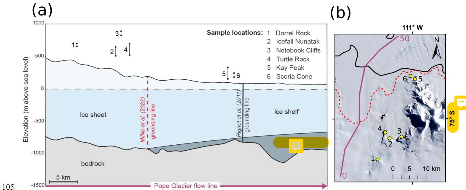
Figure 2: Relationship between nunatak elevation, bedrock and ice sheet topography (a) Cross-section transects showing modern ice surface elevation data (line above sea level; from Reference Elevation Model for Antarctica (REMA); (Howat et al., 2019) and bedrock topography (line below sea level; from BedMachine; (Morlighem et al., 2018)). Note that the glacier flowline profile (solid purple line in panel b) is >10km from the sample sites; elevation range markers on the cross-section represent the highest and lowest elevation sample at each site (m asl) (Johnson et al., 2020) and are displayed at points approximately adjacent to flowline on the right hand panel. (b) Landsat-8 true colour composite (432) image showing location of Pope Glacier flowline with distance downstream from arbitrary starting position. Profile is displayed in the cross section above. Elevation range markers on the cross-section (a) are displayed as yellow dots approximately adjacent to flowline on panel b. Landsat-8 image courtesy of the U.S. Geological Survey; https://doi.org/10.5066/P9OGBGM6 .
