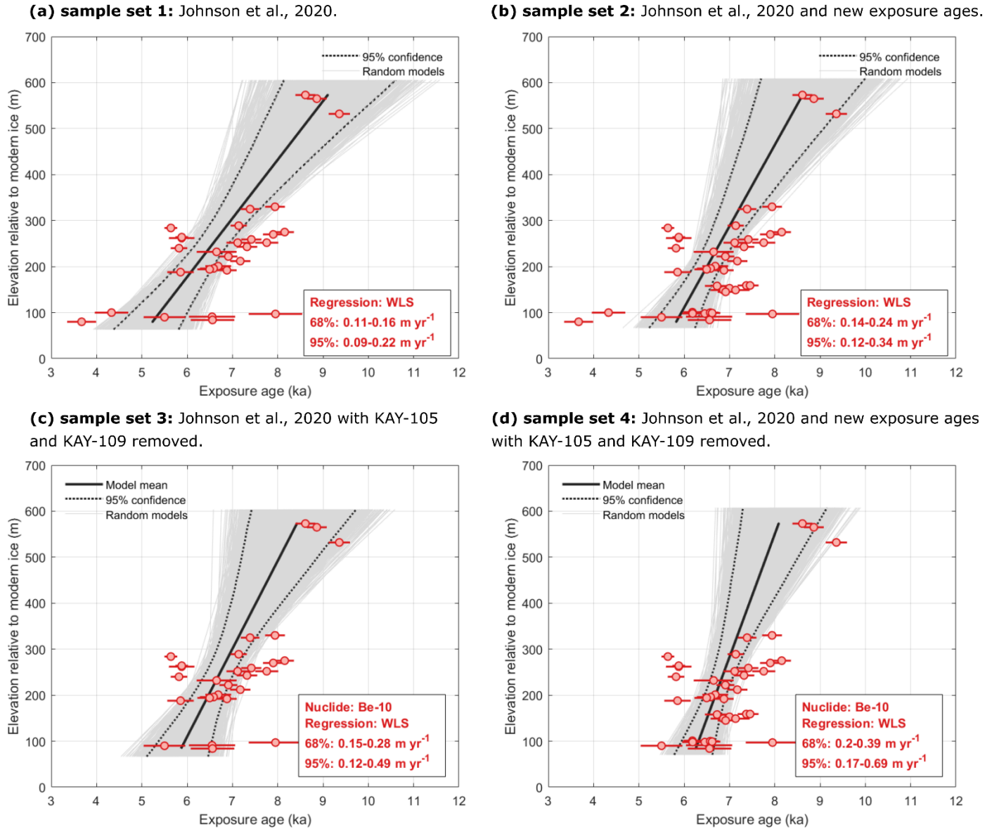
Figure B2: Linear Regression Transect of ice surface thinning generated with iceTEA: Linear regression transects showing (a) the original sample set of Johnson et al. (2020), (b) incorporating new data from Scoria Cone, (c) removing young ages identified as outliers and (d) incorporating new data from Scoria Cone as well as removing young ages identified as outliers. Black solid line is 'best fit' averaged from 5000 Monte Carlo simulations. Dotted black lines represent 95 % confidence intervals. Exposure ages displayed as red circles with internal uncertainties.
