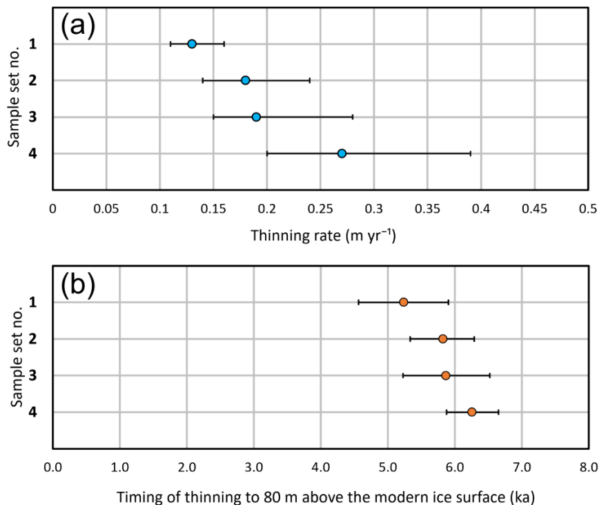
Figure 5: Thinning rates and age constraints from linear regression analysis. (a) range in thinning rates (m yr -1 ) compiled from linear regression histograms (Fig. B1) and (b) uncertainty range in best fit timing of thinning to 80 m above the modern ice surface (ka) calculated for each of the different input data to the linear regression Monte Carlo simulation (Fig. B2). Blue circles in (a) represent the median thinning rate and orange circles (b) represent the endpoint of the best fit thinning line. Error bars represent 68 % confidence interval uncertainty estimates in plot (a) and 95 % confidence interval uncertainty estimates in plot (b). The sample set no. indicates the four different age datasets used for linear regression analysis, which are described in the text above (section 3.1). Note plot b, sample sets 1 and 4 linear regression best fit end ages correspond to the linear regression transects displayed in Figure 6.
