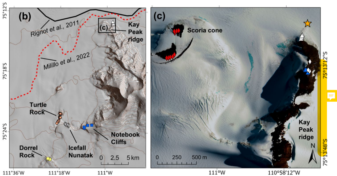
Figure 1: Location of the study area in the context of Mt Murphy and the wider ASE. (a) ASE area map displaying regional ice streams, ice velocities (Mouginot et al., 2012) overlaid on Reference Elevation Model of Antarctica (REMA) (Howat et al., 2019) regional bathymetry (Arndt et al., 2013), 2011 grounding line (black line; Rignot et al., 2011) and Antarctic coastline (blue; Antarctic Digital database, version 7.2). (b) Mt Murphy site map generated using REMA derived hill shade, with contours representing 100 m intervals. Locations of previous exposure ages (Johnson et al., 2020, 2008) indicated by coloured symbols shown in Fig. 1b key, also displayed are both the 2011 grounding line (same as in Fig. 1a), and most recent localised grounding line (red dotted; Milillo et al., 2022). (c) High resolution satellite imagery (732 false colour composite), DigitalGlobe Products, WorldView 2 © 2013 DigitalGlobe, Inc., a Maxar company showing scoria cone and Kay Peak Ridge. Drill site indicates subglacial bedrock core recovery by the Geological History Constraints (GHC) subglacial drilling project (Boeckmann et al., 2021).
