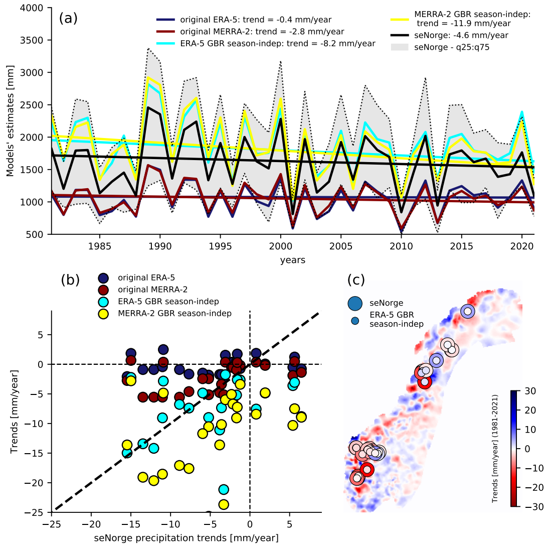
Figure S1: Precipitation (SWE) trends obtained from the original reanalyses (season-independent GBRs) compared with the seNorge model in Norway over the period 1981-2021. (a) Yearly average of models' estimates for the Norwegian glaciers of the study. (b) Comparison between reanalysis-based trends and seNorge trends for each Norwegian glacier of the study. Both reanalysis and seNorge models indicate negative trends for the majority of the analyzed glaciers. (c) Map of seNorge trends, where trends on the analyzed glaciers are highlighted.
