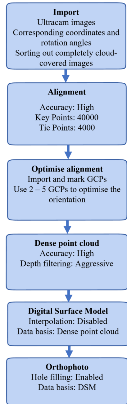
Figure 3. Flowchart illustrating the Agisoft Metashape parameter settings used to generate the winter-DSMs from Ultracam imagery.
