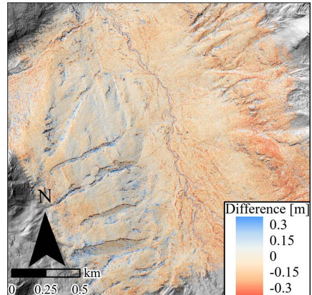
Figure 9. Difference calculation of the DSMs around the Schürlialp derived from Ultracam data and UAS in 2021.
