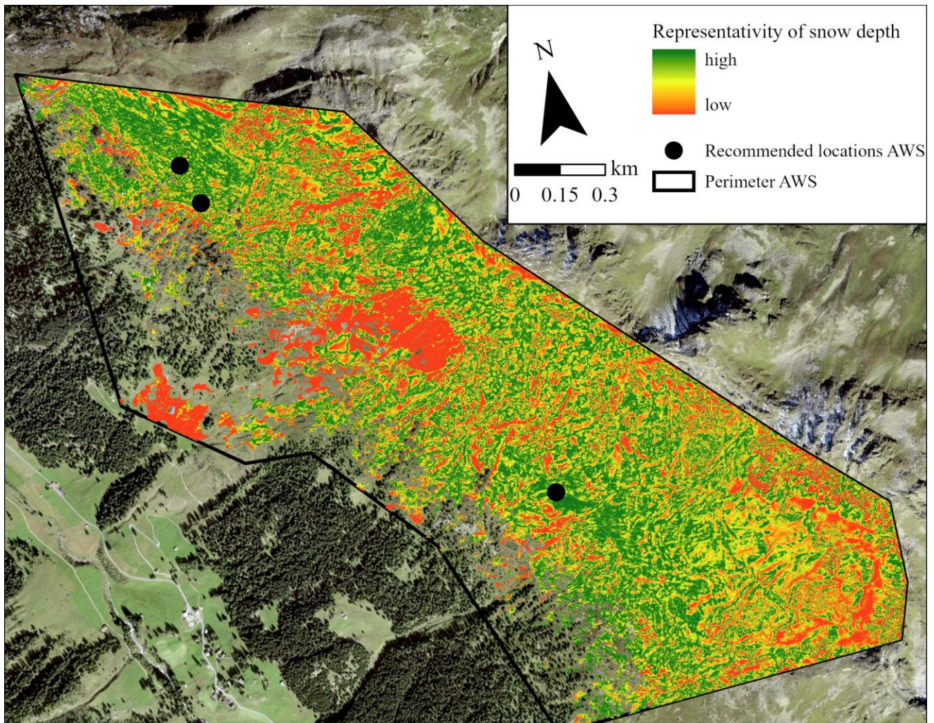
535 Figure 17. Representativity of punctual snow depth measurements (possible locations for AWS) for the entire perimeter (black polygon) derived from airplane snow depth maps. Black circles symbolise predefined locations for the AWS. The south location was finally selected due to its high representativity (dark green), low avalanche danger and flat terrain for the new AWS Lukschalp (map source: Federal Office of Topography).
