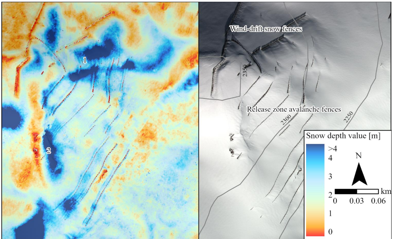
515 Figure 15. Snow depth distribution and corresponding orthophoto around avalanche fences at the Grüniberg, captured by the Ultracam 520 flight on the 16 th of March 2019. The numbers 1 and 2 indicate buried avalanche fences with snow depths exceeding 5 m.
