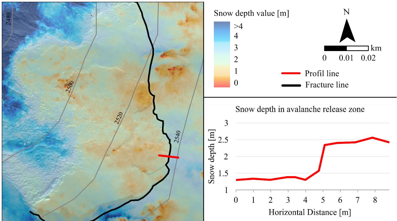
Figure 14. Overview of the snow depth distribution of the release zone of a slab-avalanche close to the Börterhorn (Dischma Valley) captured by the Ultracam in 2019; the red line symbolises a height profile showing the course of snow depth values vertical to the fracture line; the prominent difference in snow depths indicates the release height of around 0.95 m.
