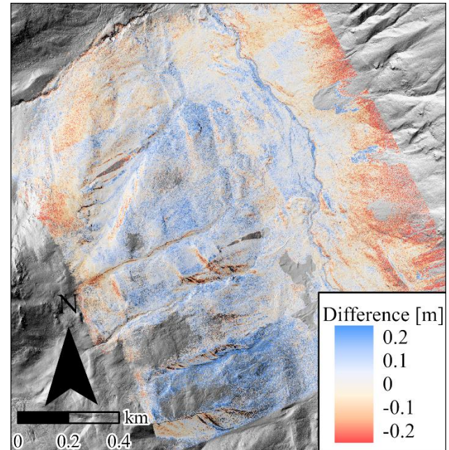
Figure 8. Difference calculation of the DSMs around the Schürlialp derived from Ultracam data and UAS in 2018.
