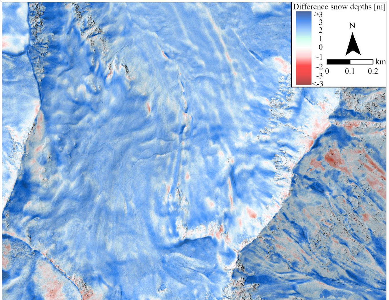
Figure 12. Difference calculation of the snow depth maps 2019 and 2020 during peak of winter in a small catchment (3 km 2 ) close to Börterhorn. Black pixels symbolize No Data values.
