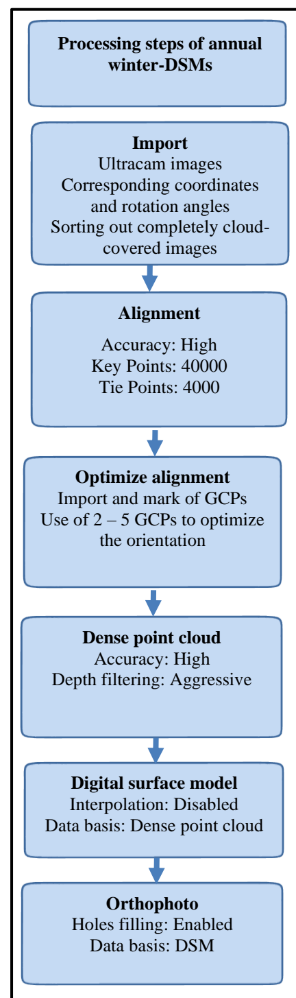
Figure 3. Flowchart illustrating the workflow generating the winter-DSMs on the basis of Ultracam images.
