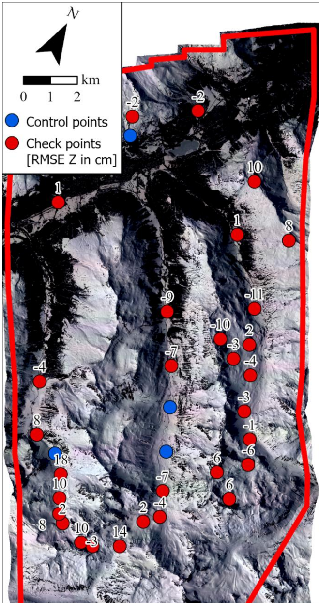
Figure A1. Overview of the distribution of ground control points (blue) and check points (red) with the corresponding RMSE Z values. Background shows the orthophoto from 2020.
