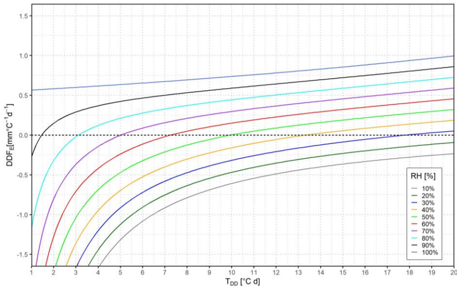
625 Figure 8 Latent Heat component ( DDF_E ) for selected relative humidity [%], degree-days [ ^{\circ}\text{C d} ] and u = 1 \text{ m s}^{-1} Note: These values are for u=1 \text{ m s}^{-1} , for a different wind speed these values can be multiplied for desired wind speed. Air density values are assumed at an elevation of 0 m a.s.l.
