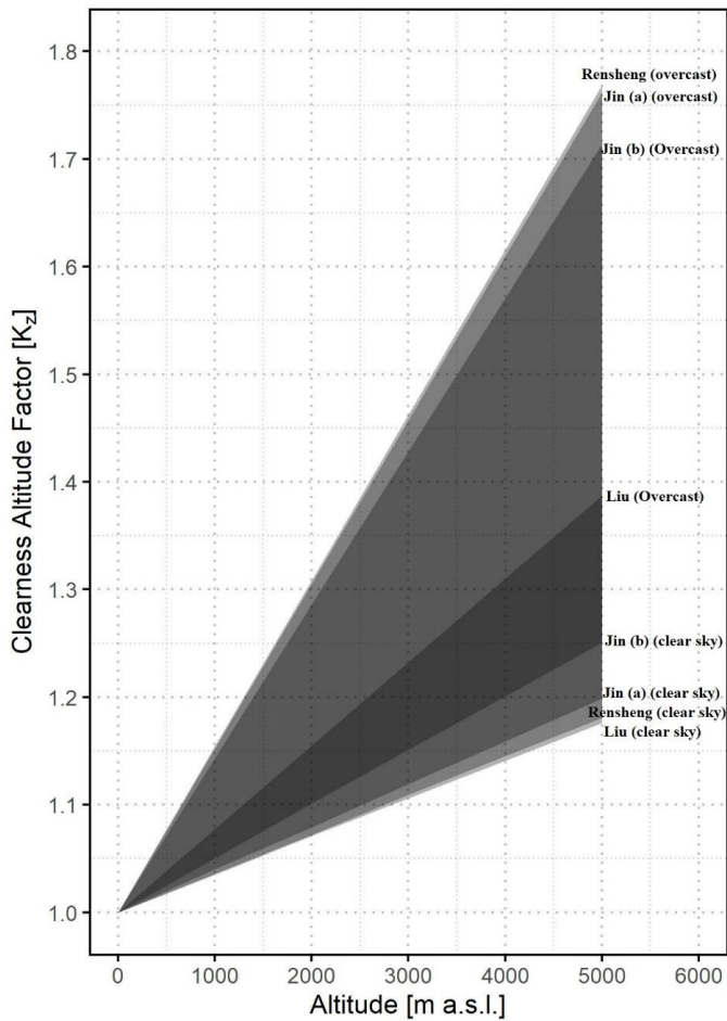
Figure 4. Clearness altitude factor K_z for different altitudes ranges, based on different models presented in equations (14 – 17, i.e. Jin (a), Jin (b), Rensheng, and Liu) for latitude 45^\circ where applicable
