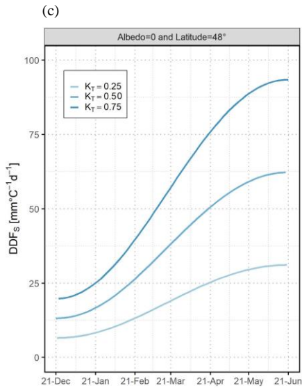
Figure 5 Variation of solar radiation based DDFs for a degree-day value of 1°C d for (a) different latitudes under constant snow albedo and clearness index; (b) snow albedos under constant latitude and clearness index; (c) different clearness indices under constant latitude and snow albedo – The latitude = 48° corresponds to the location of Brunnenkopfhütte test site.
