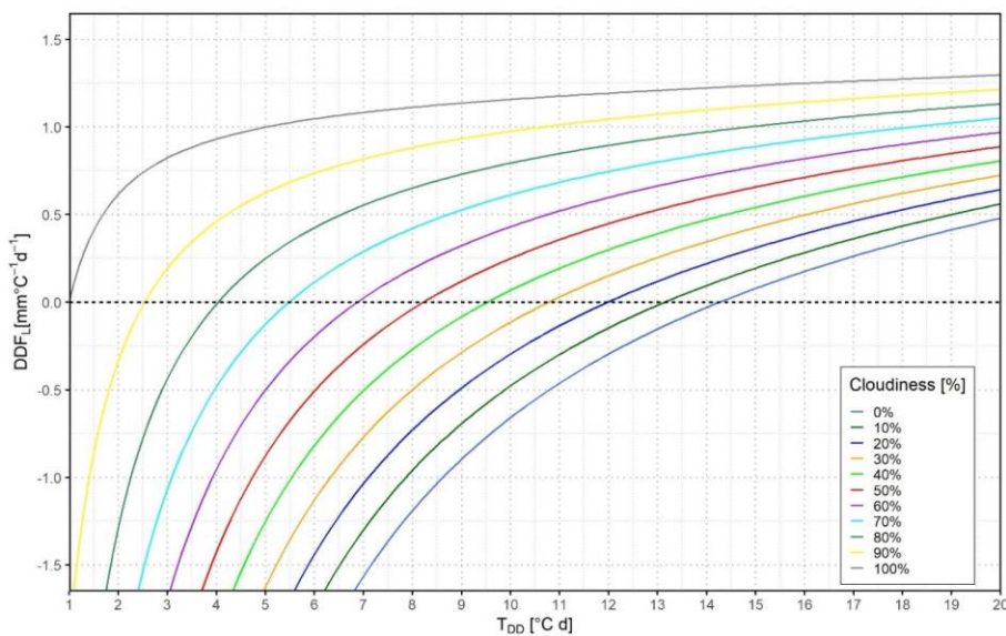
550 Figure 6 Longwave Radiation component ( DDF_L ) for selected cloudiness [%] and degree-days [°C d]
