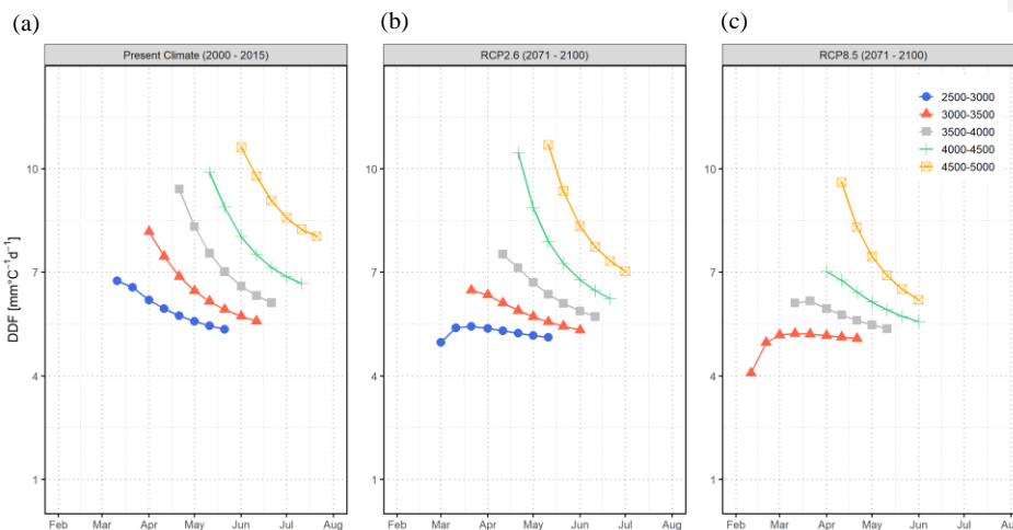
Figure 12 (a) DDF estimates for a temperature-index modelling in present climate; (b) Influence of climate change – 2071 – 2100 under RCP2.6; (c) Influence of climate change – 2071 – 2100 under RCP8.5
