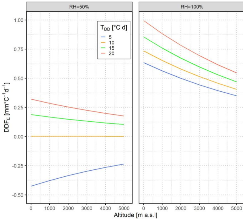
630 Figure 9 Variation of latent heat component ( DDF_E ) depending on altitude for different relative humidity values and degree-days (note: u = 1 \text{ m s}^{-1} )
