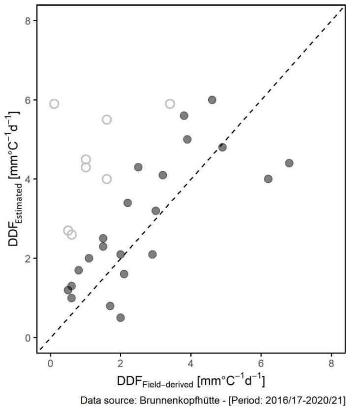
Figure 11 Comparison of field-derived vs simulated (energy flux based) 10-daily DDF for the Brunnenkopfhütte test site (period: November 2016 – May 2021) – Hollow points represent DDFs during periods with new snow events
