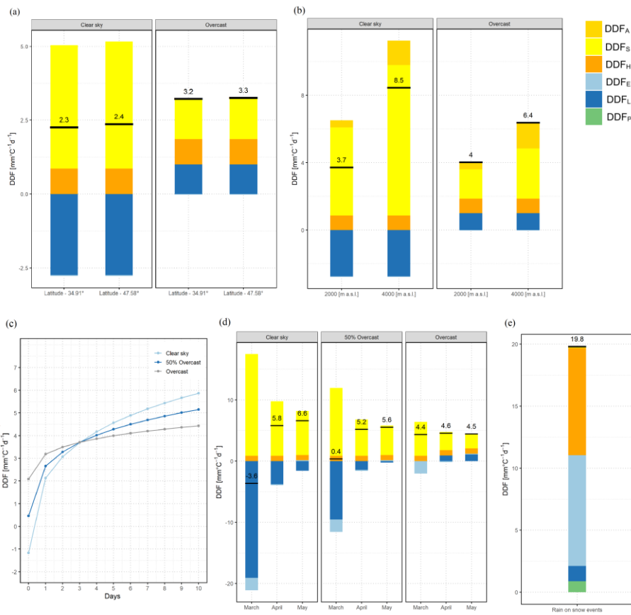
760 Figure 10 Influence of (a) latitude; (b) altitude; (c) albedo; (d) season; (e) rain on snow events – on the DDF under clear sky and overcast conditions
