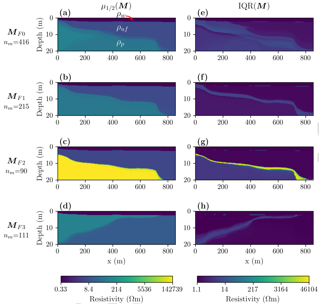
Figure 7. CE6 Inversion results for the Drew Point data set illustrated as summary statistics for all obtained models M_{F0} and for three model families M_{F1} , M_{F2} , and M_{F3} as found by cluster analysis. (a–d) Median and (e–h) interquartile range models. For each M_{Fi} , n_m represents the number of models in the corresponding ensemble.
