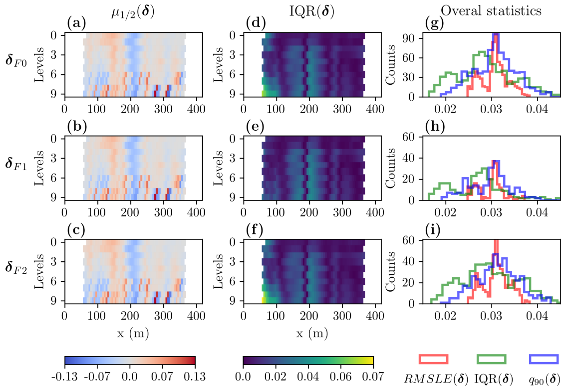
Figure 3. Summary statistics of the residuals for the Bykovsky data set corresponding to all models \delta_{F0} and for the two clustered families \delta_{F1} and \delta_{F2} . a-c) Median and d-f) interquartile range calculated in a pixel-wise fashion. g-i) Histograms illustrating the overall distribution of different statistical measures including RMSLE(\delta) , IQR(\delta) , and q_{90}(\delta) .
