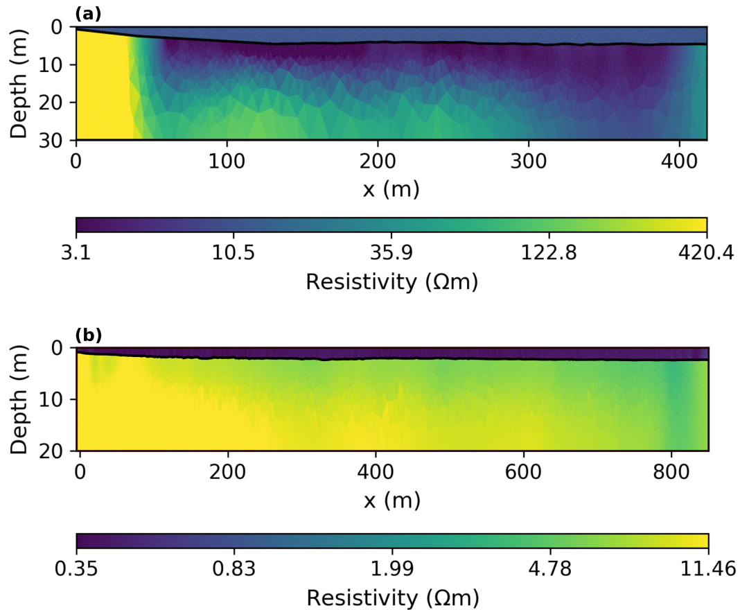
Figure A1. Smooth inversion models for (a) the Bykovsky and (b) Drew Point data sets. To enhance resistivity contrast in our ERT models presented in (a) and (b), we limited the lower and upper resistivities considering quantiles 0.04 and 0.96, respectively.
