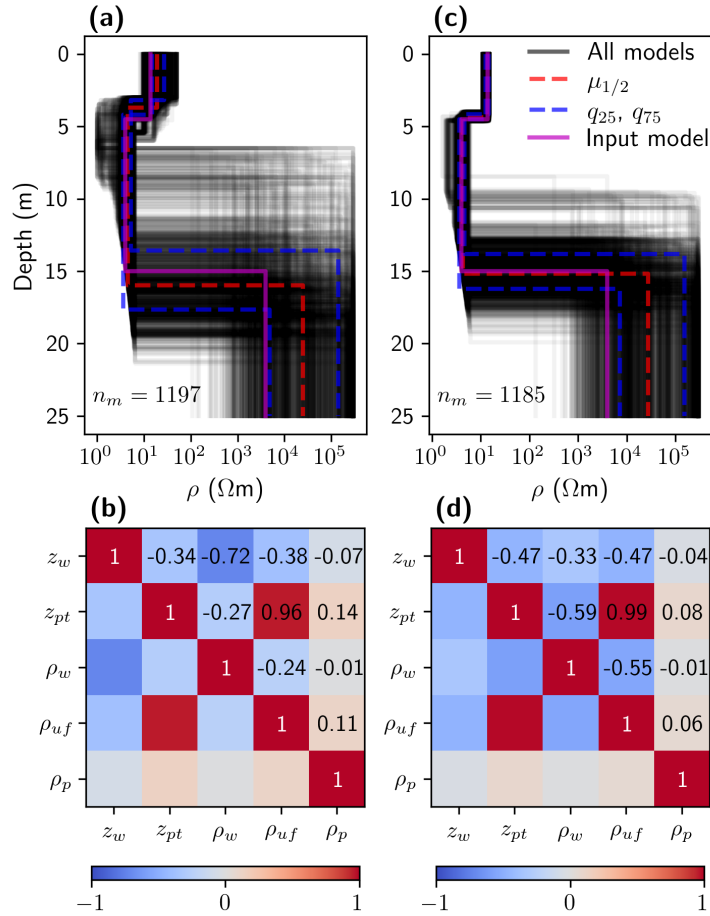
Figure 4. 1D inversion results of synthetic data for 1D subsurface scenarios developed for the Bykovsky field site. a) Ensemble with n_m model solutions and b) the corresponding symmetric correlation matrix for scenario 1 (water layer parameters with large freedom during inversion), and c)-d) the same for scenario 2 (with constrained z_w and \rho_w ). Black lines in a) and c) are plotted with transparency and, therefore, the darker areas indicate higher densities model. The numbers in b) and d) are the corresponding correlation values.
