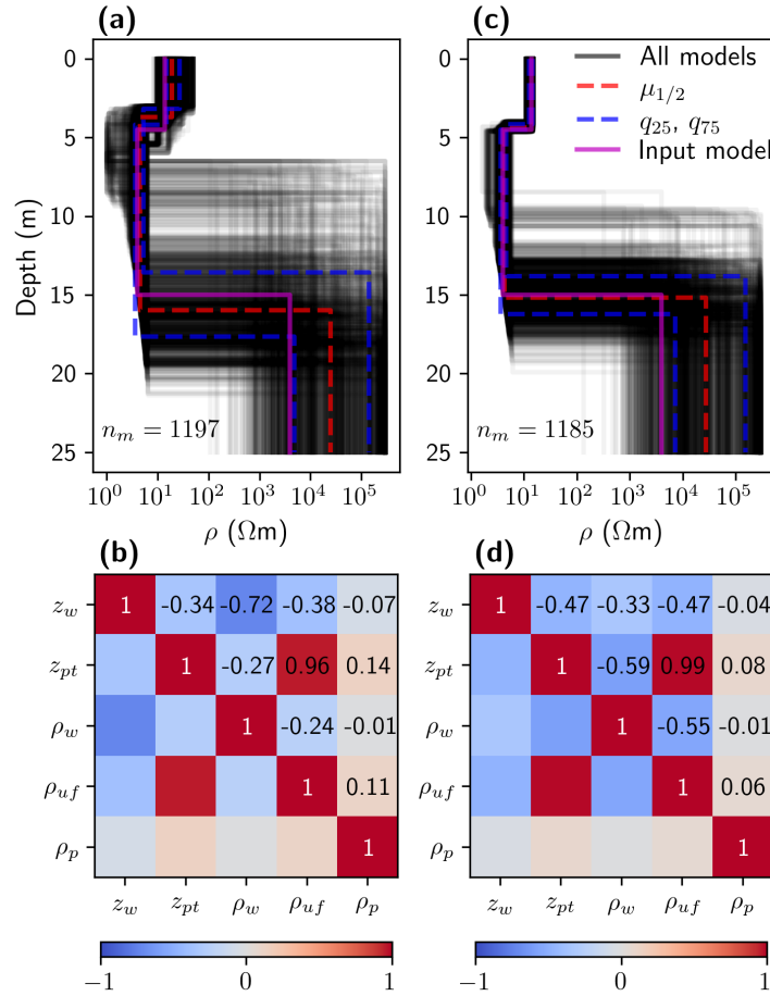
Figure 4. 1D inversion results of synthetic data for 1D subsurface scenarios developed for the Bykovsky field site. a) Ensemble of n_m model solutions and b) the corresponding symmetric correlation matrix for scenario 1 (water layer parameters with large freedom during inversion), and c-d) the same for scenario 2 (with constrained z_w and \rho_w ). Note, black lines in a) and c) are plotted with transparency and, therefore, the darker areas indicate higher densities model. Each ensemble contains n_m model solutions. The numbers in b) and d) are the corresponding correlation values.
