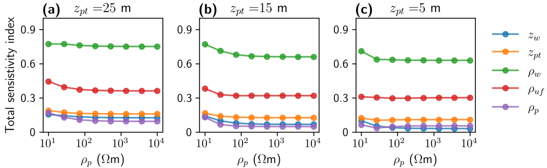
Figure 6. Global sensitivity results for the Bykovsky field site considering different 1D model scenarios with an IBPT at a depth of a) 25 m, b) 15 m, and c) 5 m.
