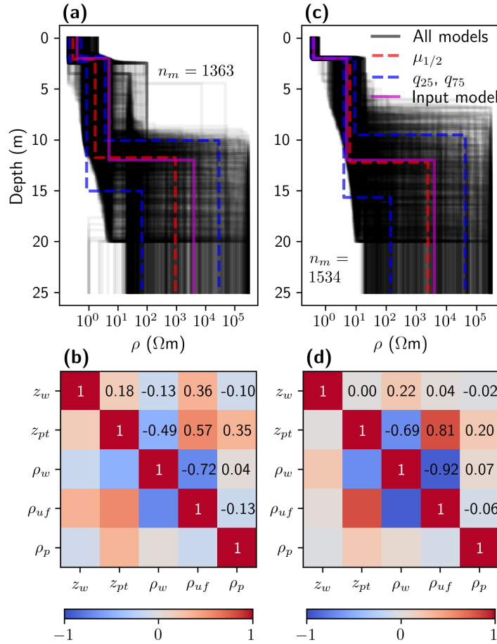
Figure 9. 1D inversion results of synthetic data for 1D subsurface scenarios developed for the Drew Point field site. a) Ensemble of n_m model solutions and b) the corresponding symmetric correlation matrix for scenario 1 (water layer parameters with large freedom during inversion), and c-d) the same for scenario 2 (with constrained z_w, \rho_w, and \rho_{uf} ). Note, black lines in a) and c) are plotted with transparency and, therefore, the darker areas indicate higher densities model. Each ensemble contains n_m model solutions. The numbers in b) and d) are the corresponding correlation values.
