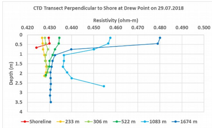
Figure 1. CTD profiles taken along our ERT transect at our Drew Point field site. Note that the line colors indicate the distance from the shoreline.
