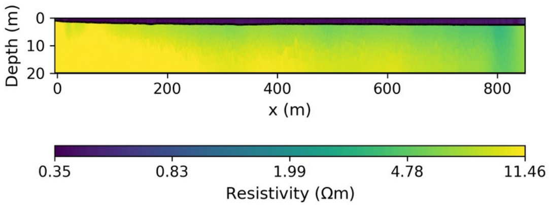
Figure 2. Smooth inversion result for our Drew Poin data set constraining the water layer.
