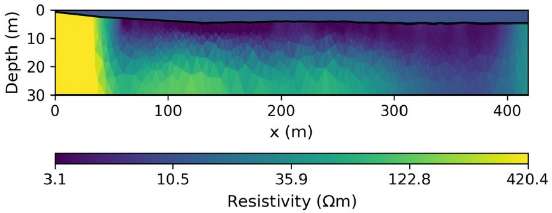
Figure 1. Smooth inversion result for our Bykovsky data set constraining the water layer.
