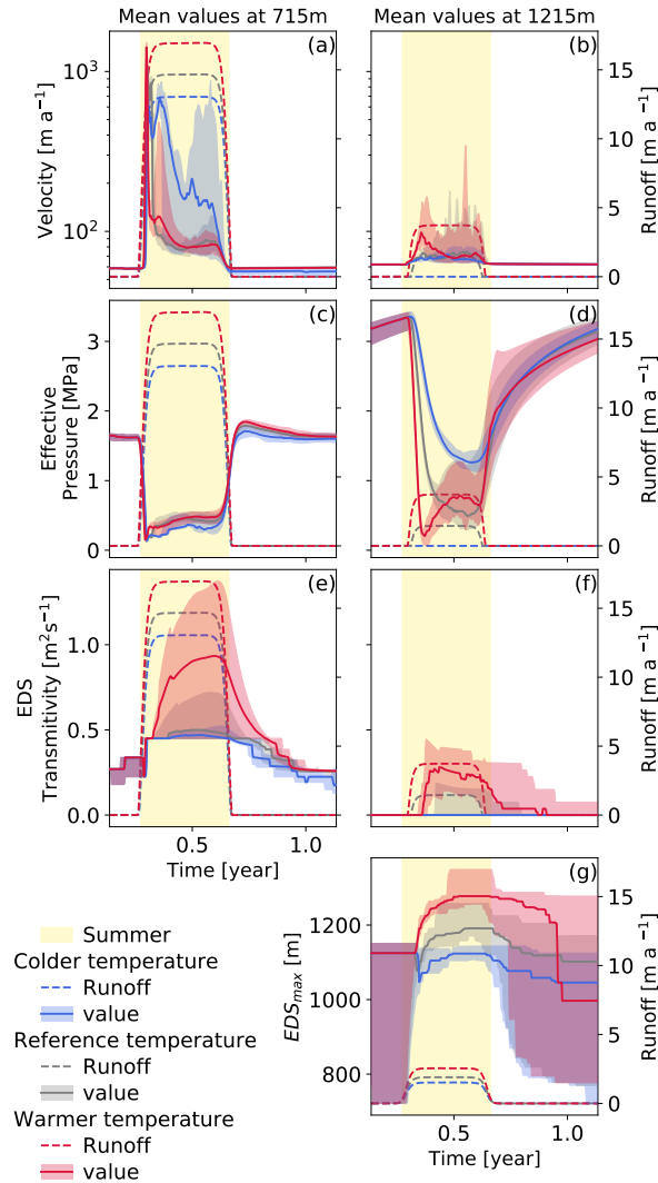
Figure 7. Evolution of the velocity (a-b), effective pressure (c-d) and efficient drainage system transmittivity (e-f) at two different altitudes. Evolution of the maximum height of the active EDS (g). Every panel shows the reference simulation in grey, the higher intensity melt season in red and the lower intensity melt season in blue. The same colour scheme is used for the runoffs which are shown as dashed lines and are referenced on the right axis. The yellow shading correspond to the fixed duration summer as defined in Sect. 2.3
