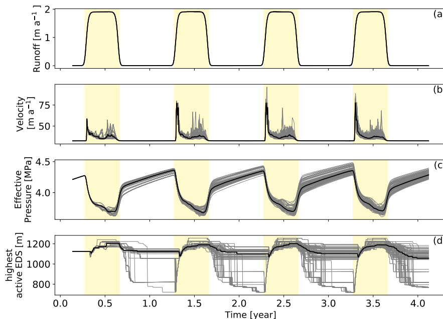
Figure 2. Evolution of the surface runoff (a), ice velocity (b), effective pressure (c) and highest active efficient drainage system node (d) averaged . All panels show spatial means over the whole domain. The yellow shading represent the summer period while every grey line corresponds to one member of the ensemble of simulations and the black thick line represent the median of the ensemble.
