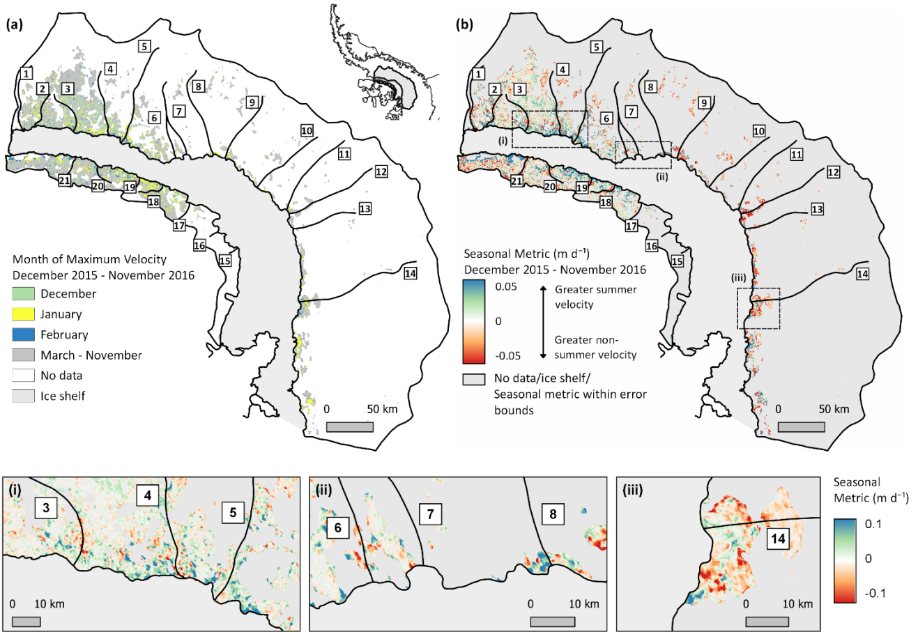
470 Figure C2 - Same as Fig. 3 but showing spatially resolved patterns of seasonal ice-flow as observed between December 2015 and 475 November 2016. (a) shows the month of maximum velocity ( v_{time} ); (b) the calculated velocity anomaly ( v_{anom_{SAR}} ). In (b), positive velocity anomalies (blue) indicate summertime speed-up; negative (red), greater velocity during non-summertime months. Dashed boxes denote the location of the inset boxes (i-iii). See also Figs. C1, C3-C4.
