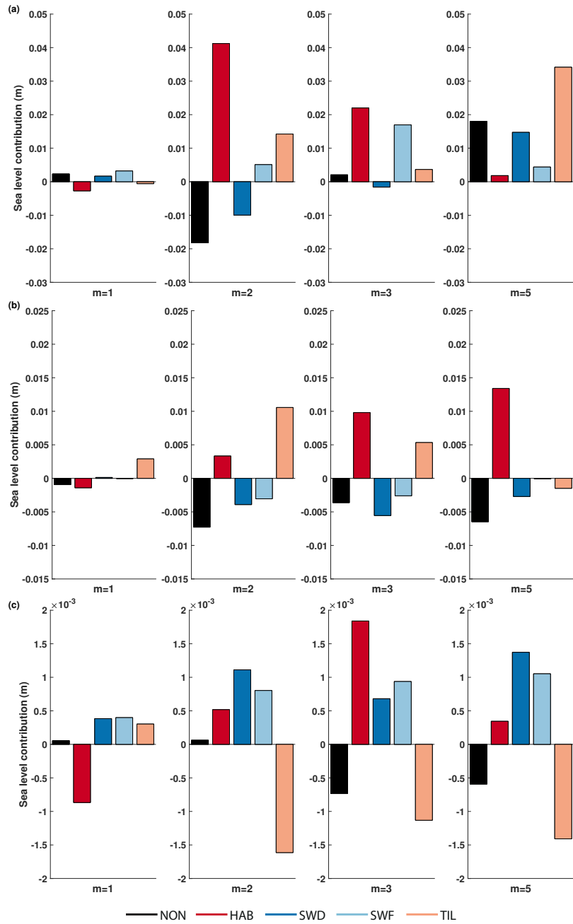
Figure 9. Sea level contribution according to HadGEM2-RCP8.5 for different basins, different values of m in the sliding law and subglacial hydrology: Pine Island and Thwaites Glacier-glaciers (a), Wilkes basin-Land (b), Enderby Land (c). Color bars represent the different subglacial models (Table 2).
