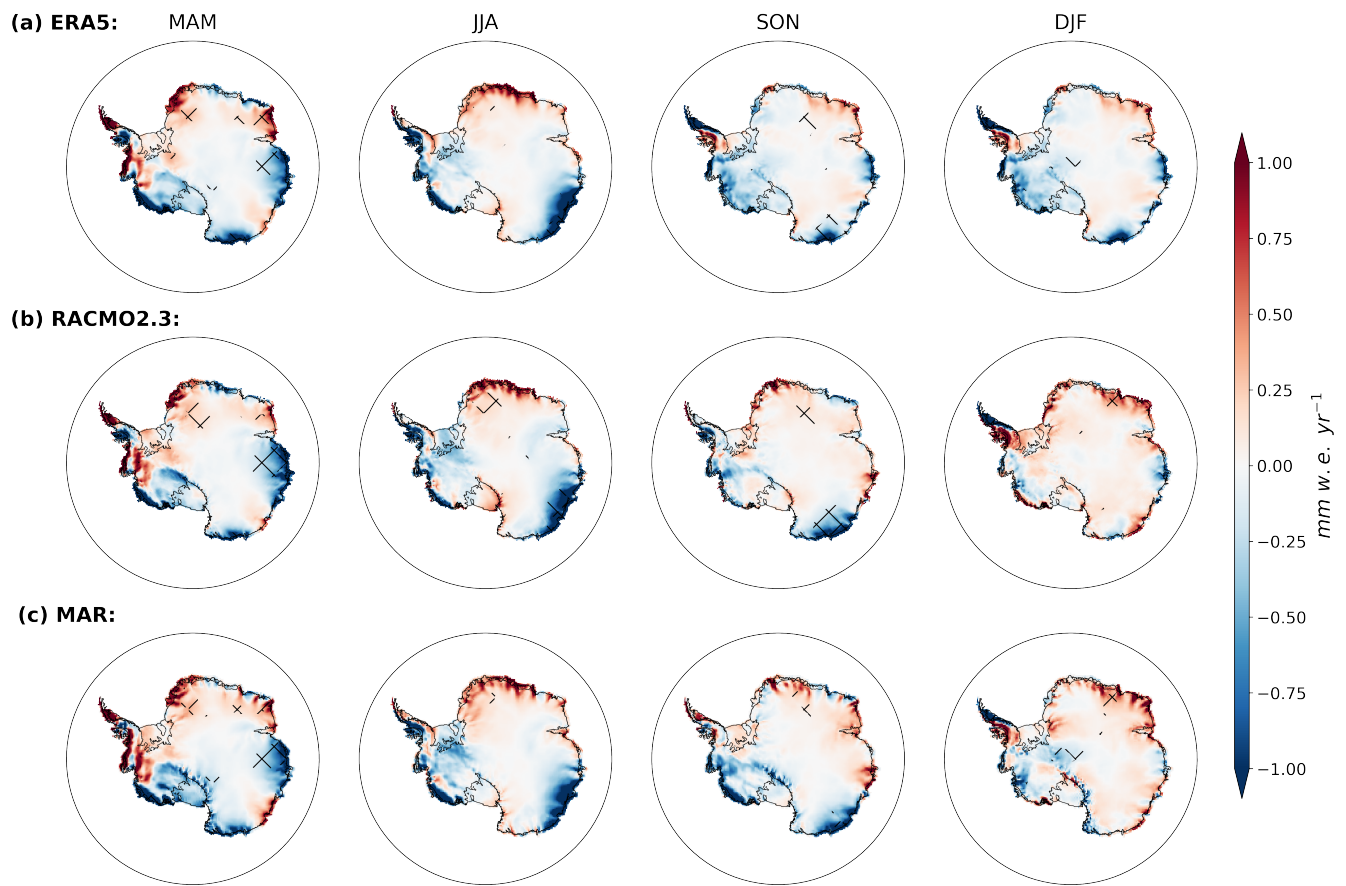
Figure A2. 1979-2015 seasonal trend in precipitation from ERA5 (a), RACMO2.3 (b), and MAR (c).
