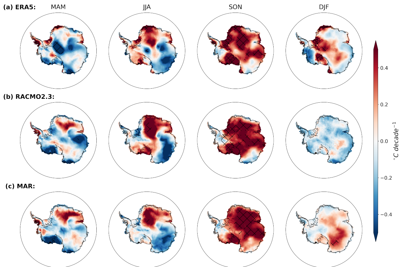
Figure A1. 1979-2015 seasonal trend in near-surface temperature from ERA5 (a), RACMO2.3 (b), and MAR (c).
