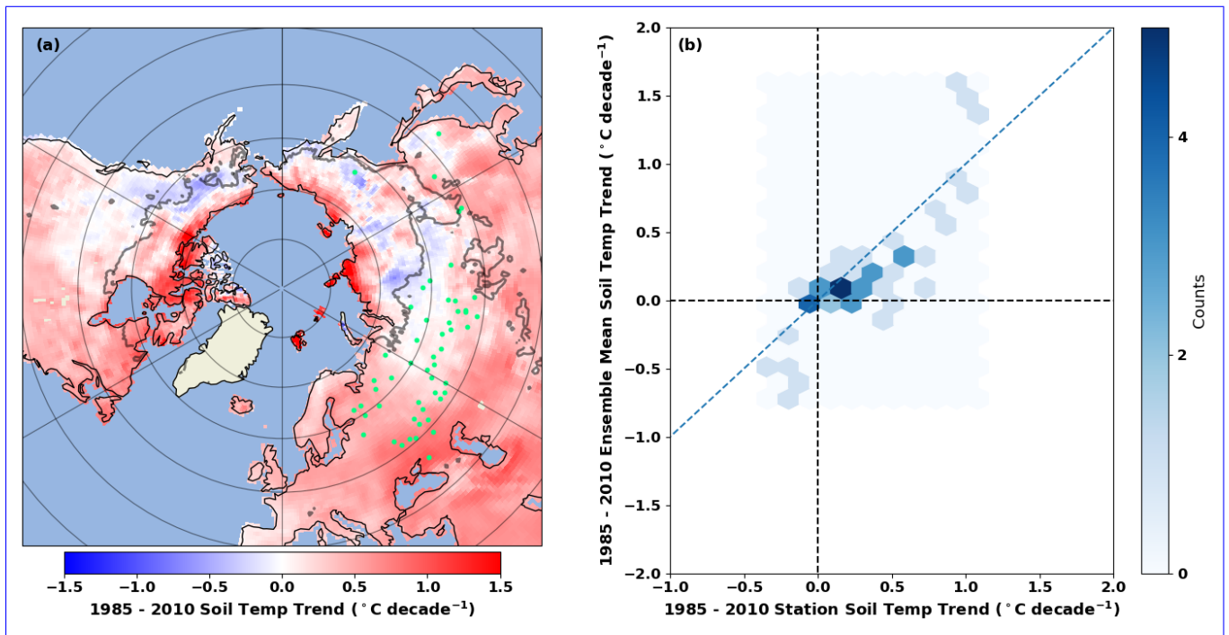
Figure 12. (a): 1985-2010 Ensemble Mean decadal soil temperature trends, near the surface, with the locations of validation grid cells included in the trend analysis shown as green dots. (b): Relationship between the near surface ensemble mean and station soil temperature trends (per decade). The black line represents the boundary of the permafrost zone (regions with at least 50% permafrost cover).
