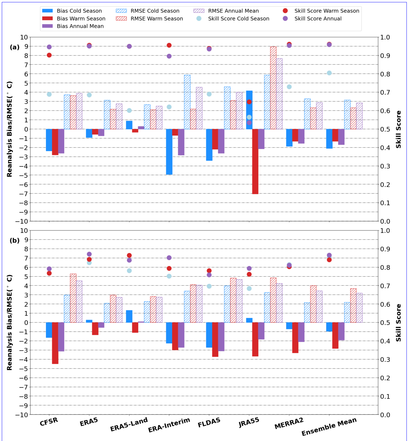
Figure 2. Bias (solid color), RMSE (hatching) and skill scores (circles) of each product the cold season (blue) ( \leq -2^{\circ}\text{C} ) and the warm season (red) ( > -2^{\circ}\text{C} ) performance of reanalysis products. The skill score is also shown over the annual cycle (purple). (a) displays the bias, RMSE and skill score for the near surface (0 cm to 30 cm) layer, while (b) displays the bias, RMSE and skill score at depth (30 cm to 300 cm). The ensemble mean is shown beside for comparison.
