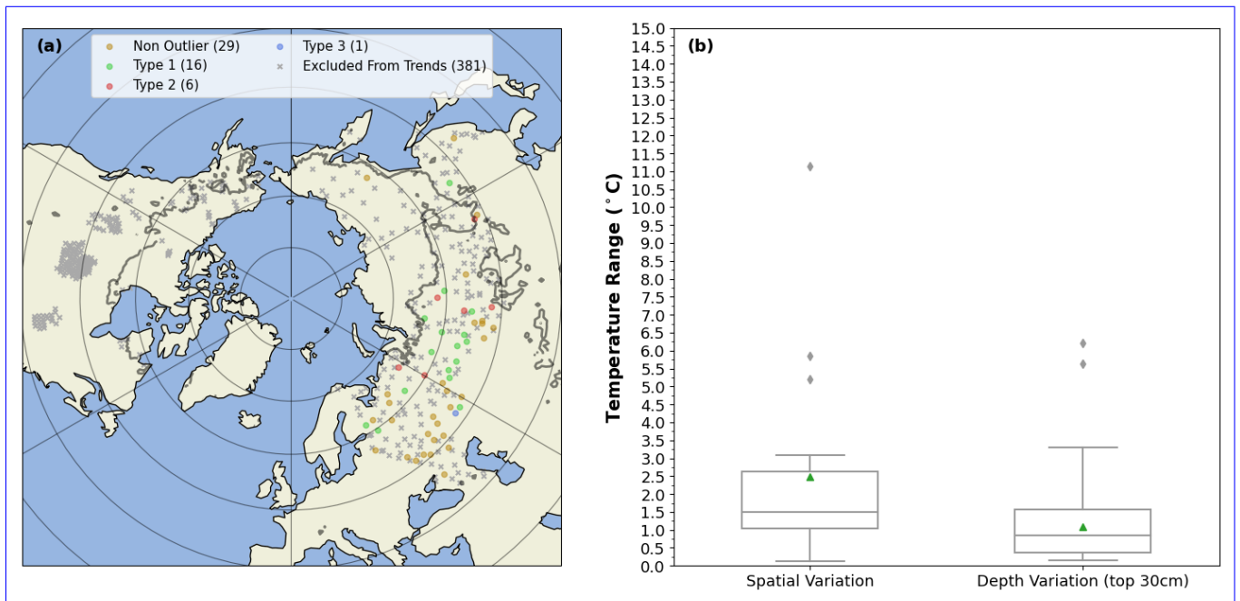
Figure 1. (a): location of the validation grid cells collocated with in situ stations in the near-surface layer. Grid cells excluded from the soil temperature trends analysis are shown as an "x". Type 1 refers to grid cells that where the ensemble mean simulates a winter minimum soil temperature that is too cold. Type 2 refers to grid cells where the ensemble mean simulates a summer maximum soil temperature that is too cold. Type 3 refers to grid cells where the ensemble mean underestimates the seasonal cycle of soil temperatures. The number in brackets beside each legend entry displays the number of grid cells in each category. The contour line encircles regions where the Obu et al. (2018) permafrost cover is at least 50 percent. (b): Impact of spatial variation and depth variation on the spread of soil temperatures in a grid cell. The mean is shown by a green triangle, and outliers are shown as grey diamonds.
