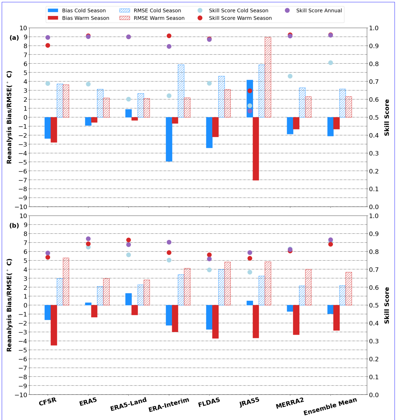
Figure 2. Bias (stippling/solid color), RMSE (hatching) and skill scores (small circles) of each product the cold season (blue) ( \leq -2^\circ\text{C} ) and the warm season (red) ( > -2^\circ\text{C} ) performance of reanalysis products. Panel A (a) displays the bias, RMSE and skill score for the near surface (0 cm to 30 cm) layer, while panel B (b) displays the bias, RMSE and skill score at depth (30 cm to 300 cm). The ensemble mean is shown beside for comparison.
