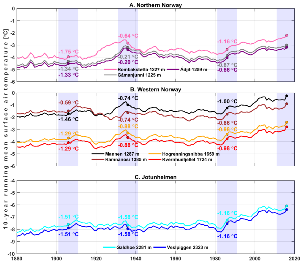
Figure A1. 10-year running mean surface air temperature (SAT 10a ) for peak elevations along each of the constructed profile in Northern and Western Norway, together with Jotunheimen. Numbers along the plot lines are mean decadal temperature offsets in the 1900s, 1930s and 1980s relative to the 2010s. Data from Hanssen-Bauer et al. (2006), Lussana (2020) and meteorological stations.
