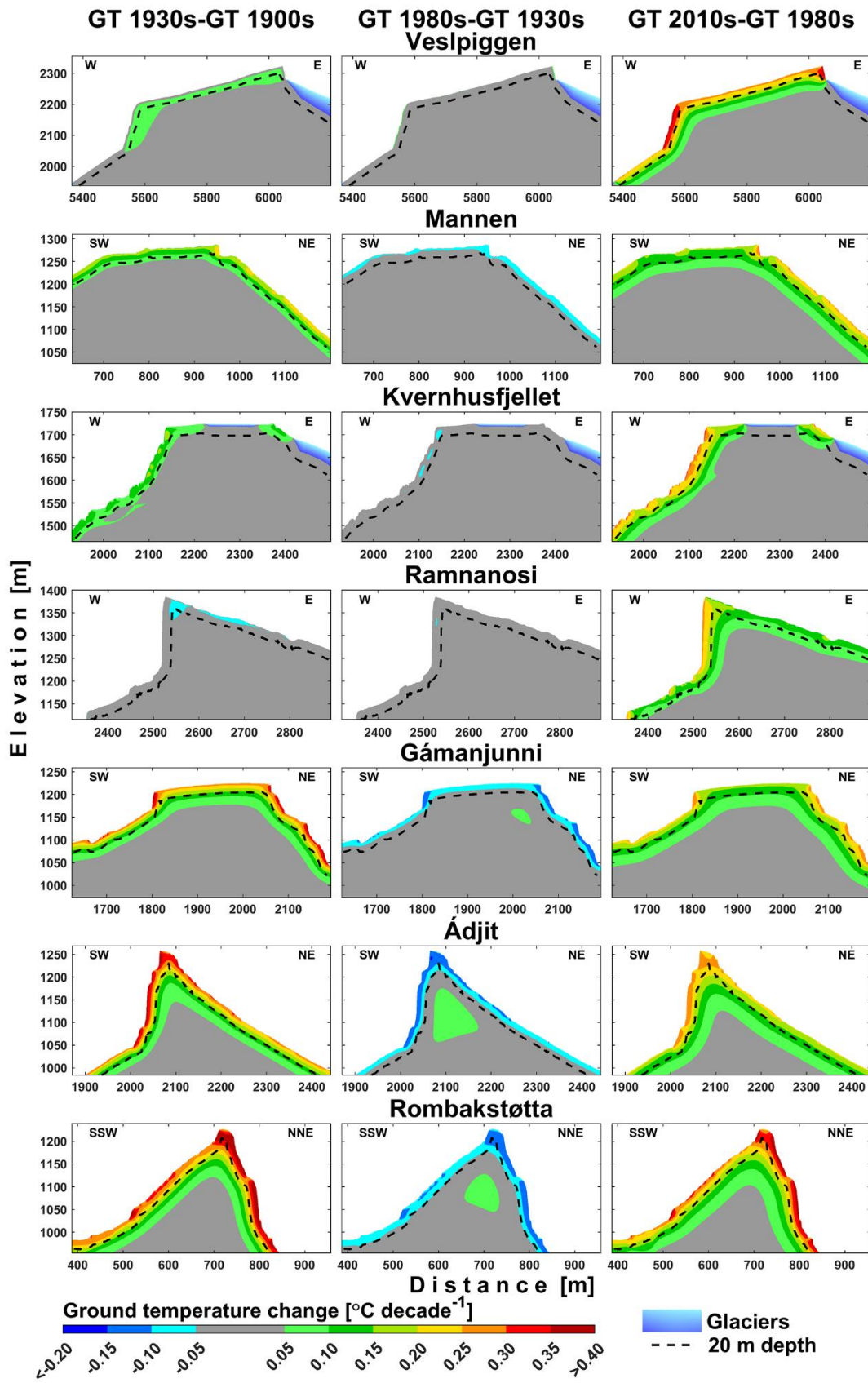
1210 Figure 7. Rate of change in 10 year mean GT for the various profiles between the following decades: (1) the 1900s and 1930s, (2) the 1930s and 1980s, (3) the 1980s and 2010s. 20 m depth is delineated by the black dashed lines.
