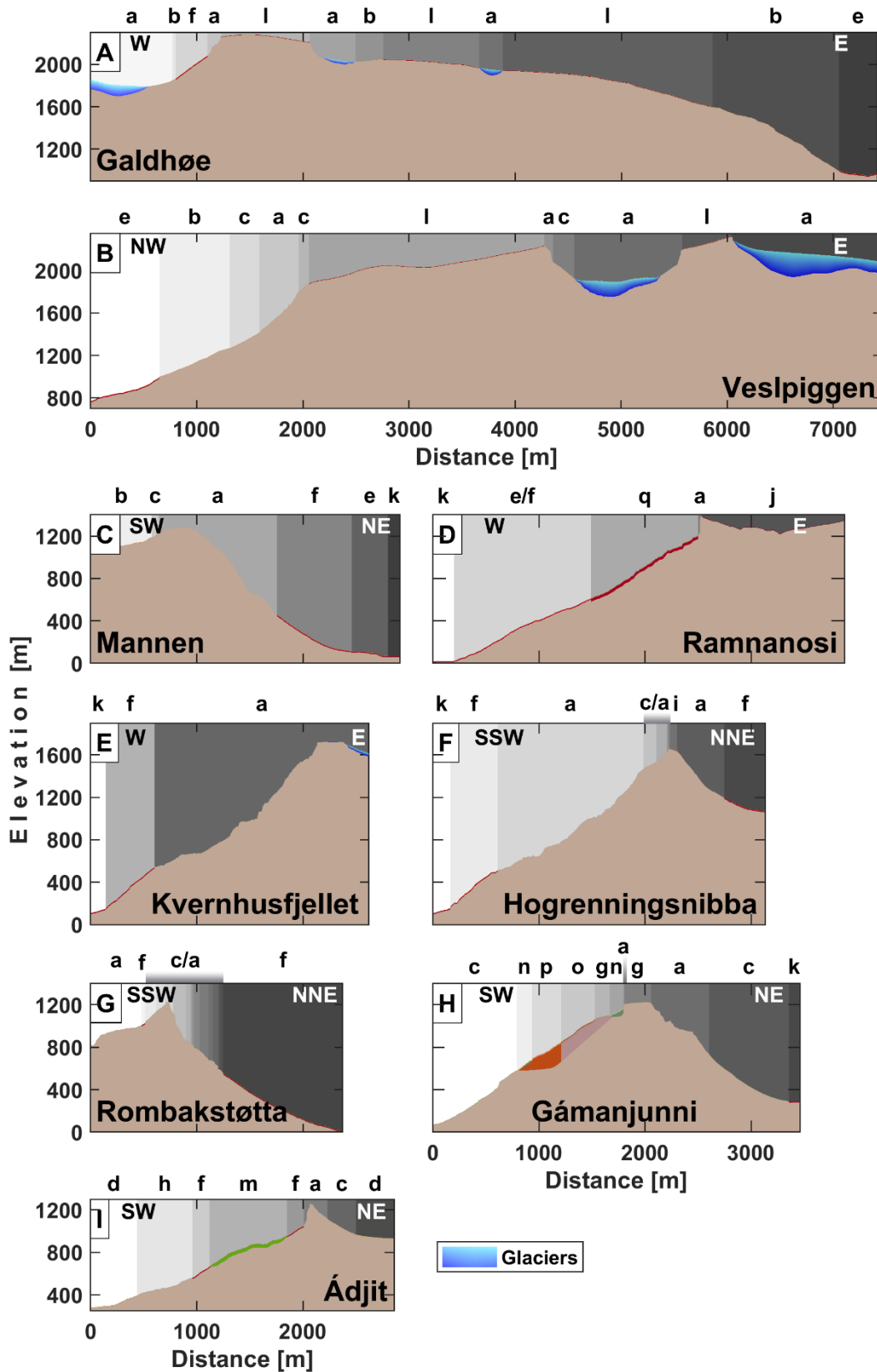
Figure 2. Slope geometry and stratigraphy. The small case letters are stratigraphy codes described in detail in Supplementary Table S1. The label “c/a” indicates alternating stratigraphy of bedrock and thin colluvium. Blue patches depict glaciers or perennial snow. Note that the meshes extend down to 6000 m below sea level and the parts below valley bottoms are not shown.
