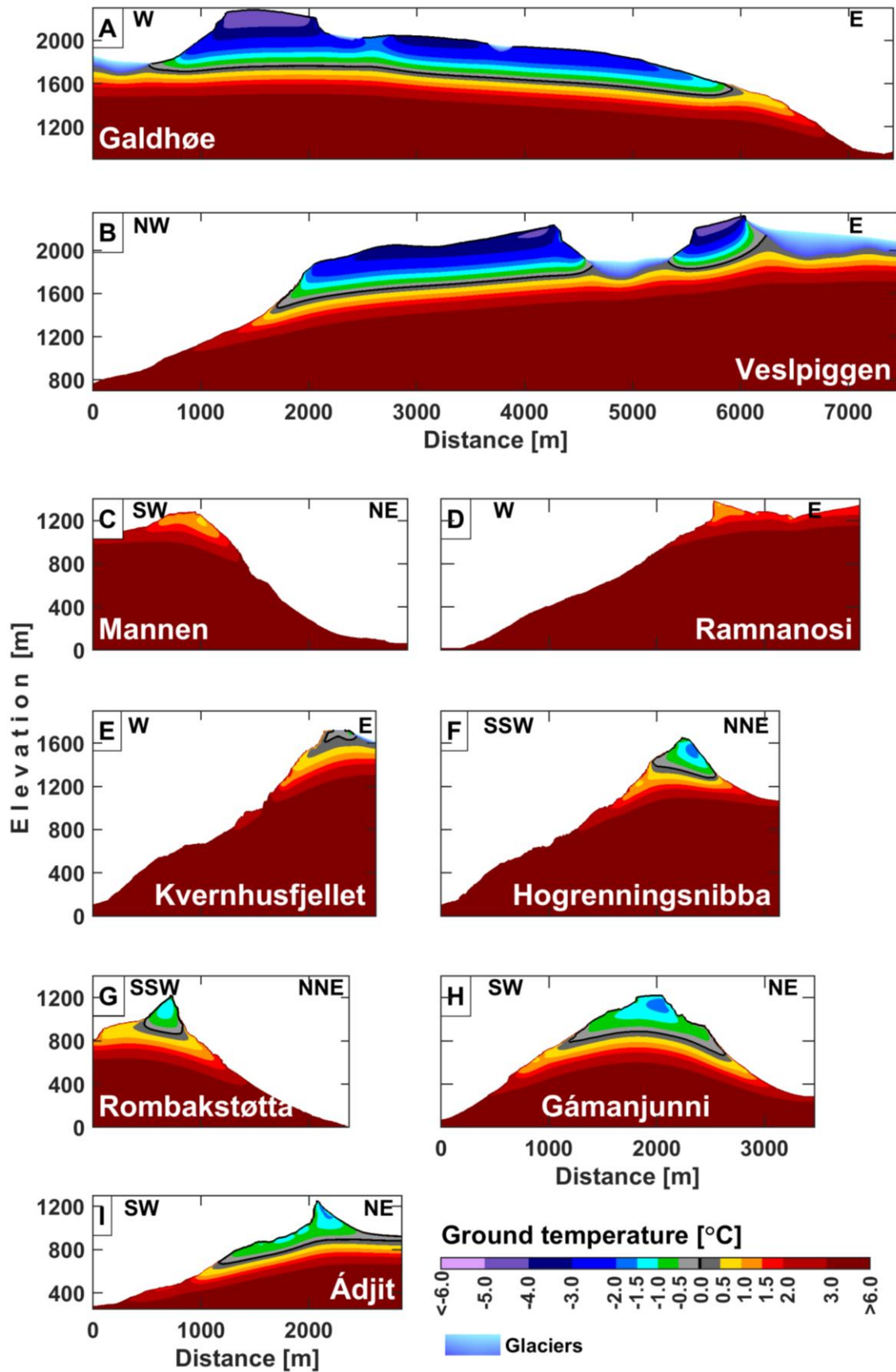
1200 Figure 4. Average annual maximum GT over the 2010s.
