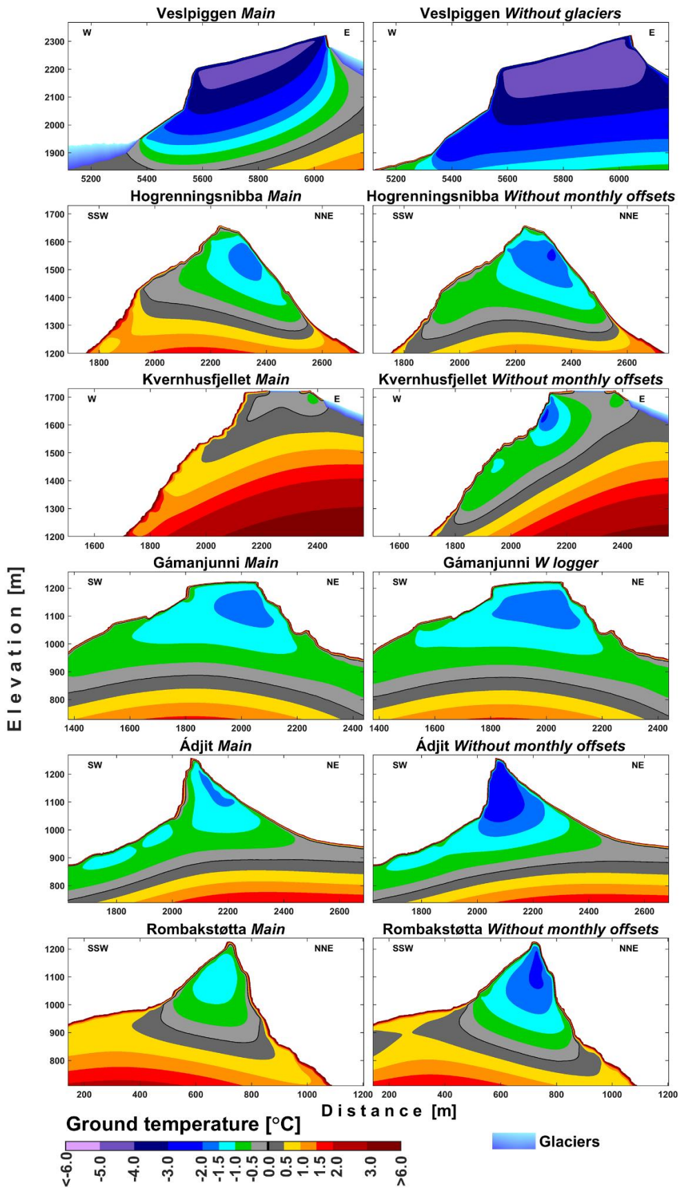
Figure 5. Average annual maximum GT over the 2010s for various simulations.
