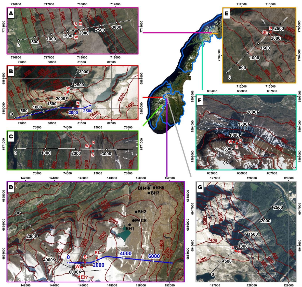
1170 Figure 1. Transects for the two-dimensional modelling. A) Gámanjuni 3, Kålfjord, B) Hogrenningsnibba (the 1175 northernmost profile/the black line) and Kvernhusfjellet (the southernmost profile/the blue line), Stryn, C) Ramnanosi, Aurland, D) Veslpiggen (the southernmost profile/the black line) and Galdhøe (the northernmost profile/the blue line), the Jotunheimen Mountains, E) Ádjit, Storfjord, F) Rombakstøtta, Narvik, and G) Mannen, Rauma. Red points with letters depict rock wall loggers in the various expositions: N=north-facing logger, S=south-facing logger, E=east-facing 1175 logger, W=west-facing logger, suffix “l”=at a lower elevation, suffix “h”=at a higher elevation. Black circles show borehole locations. Numbers along the profiles indicate distance in metres. Three geographical regions of Western, Eastern and Northern Norway are outlined by the blue lines. Map background credits: © Statens kartverk, Geovekst og kommunene. Coordinates in UTM zone 33N are shown.
