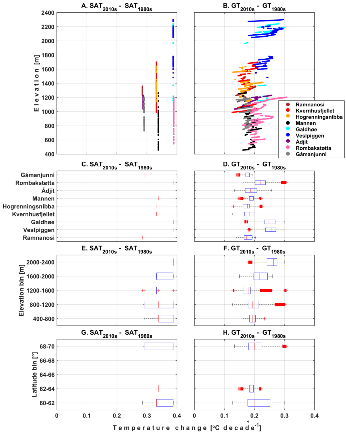
1215 Figure 8. Rates of SAT and GT change at 20 m depth between the 1980s and 2010s for all nodes below steep rock slopes (slope gradient > 60^{\circ} ). Lower subplots: Boxplots with SAT and GT rise between the 1980s and 2010s for: (C-D) every profile, (E-F) 400 m elevation bins and (G-H) 2-degree latitude bins.
