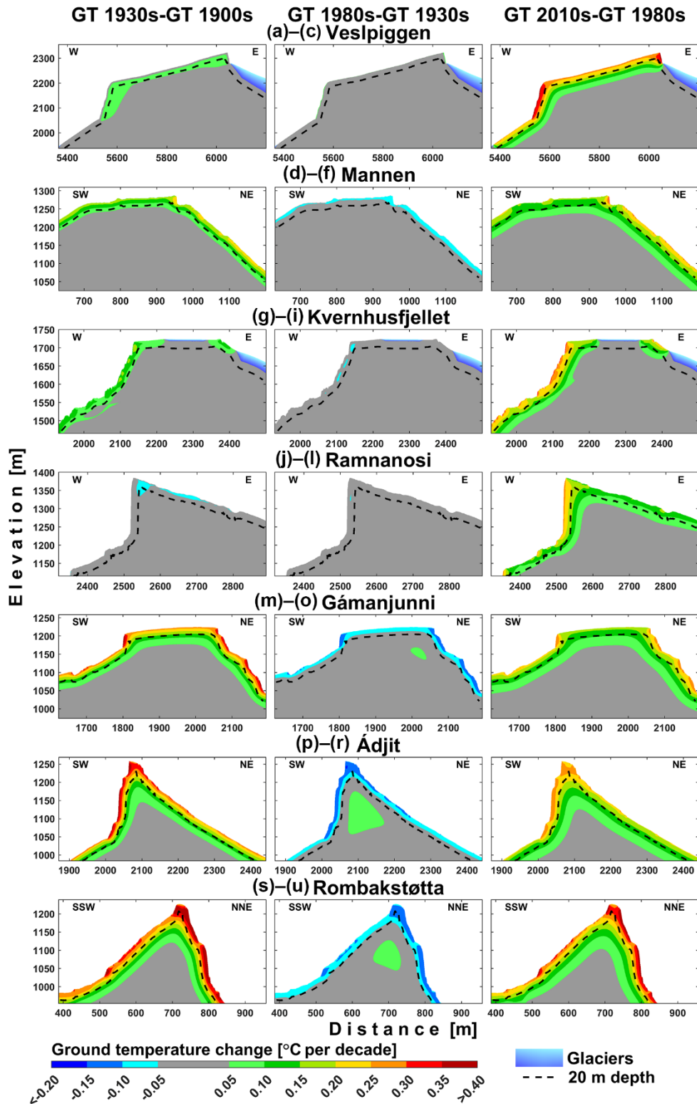
Figure 7. Rate of change in simulated 10-year-decadal mean GT-ground temperature (GT) for the various profiles between the following decades: (1) the 1900s and 1930s, (2) the 1930s and 1980s, (3) the 1980s and 2010s. 20 m depth is delineated by the black dashed lines.
