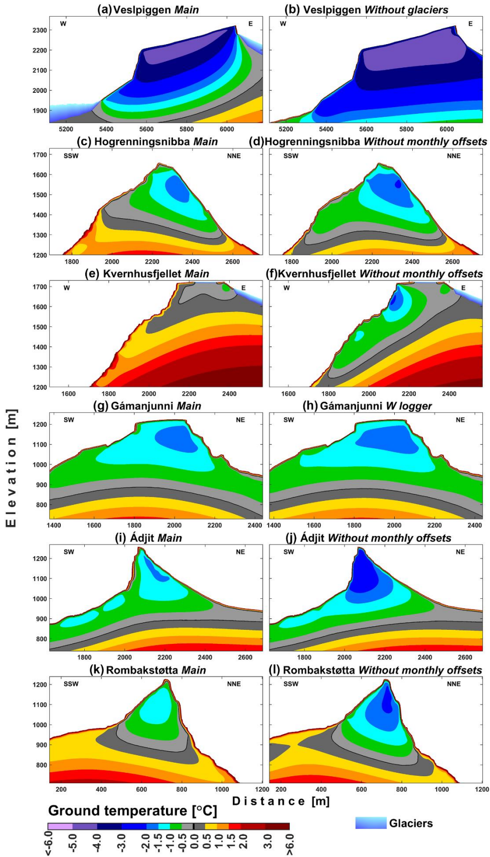
Figure 5. Simulated A verage annual maximum GT -ground temperature over the 2010s for various simulations.
