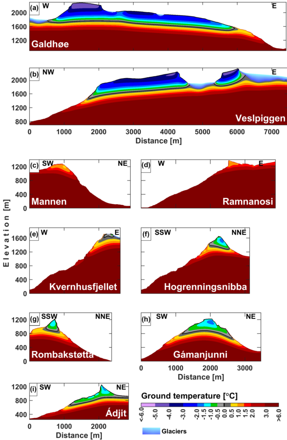
Figure 4. Simulated A verage annual maximum GT -ground temperature over the 2010s.
