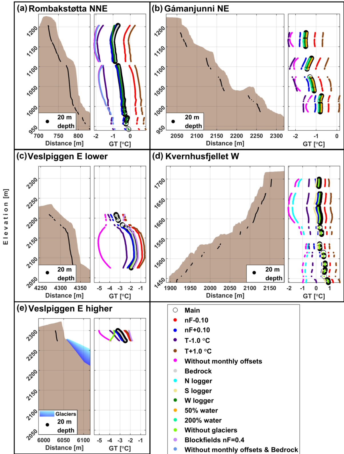
255 Figure 6. Simulated GT-ground temperature (GT) in rock walls at 20 m depth for various profiles over the 2010s. Right subplots show GT-ground temperature in nodes depicted in left subplots.
