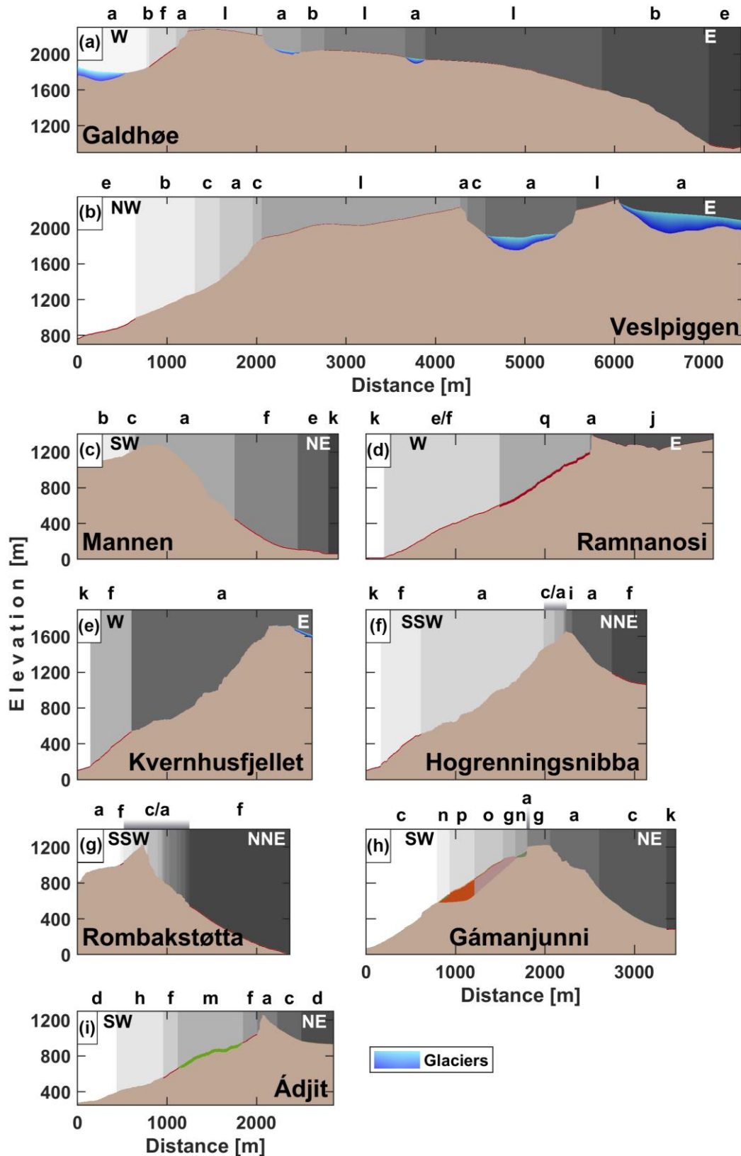
1235 Figure 2. Slope geometry and stratigraphy. The small case letters are stratigraphy codes described in detail in Supplementary Table S1. The label “c/a” indicates alternating stratigraphy of bedrock and thin colluvium. Blue patches depict glaciers or perennial snow. Different colours near the surface show various stratigraphic layers (See Supplement Table S1 for details). Note that the meshes extend down to 6000 m below sea level and the parts below valley bottoms are not shown.
