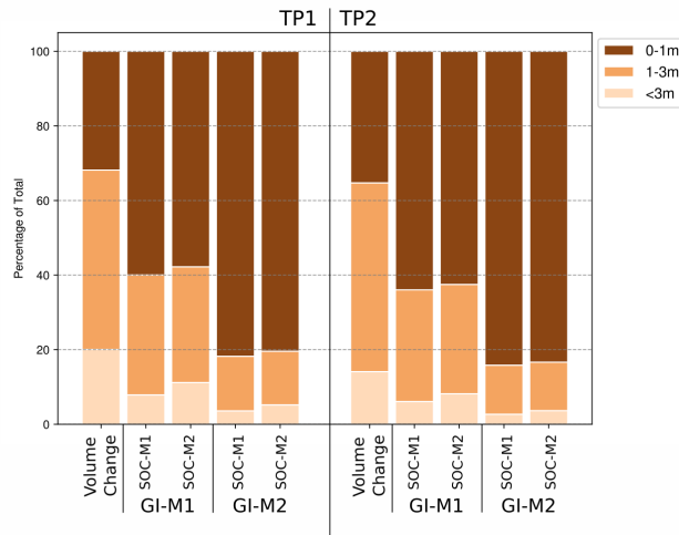
Figure 9. Mobilization of Volume and SOC separated by different depth columns in terms of percentage of total.
