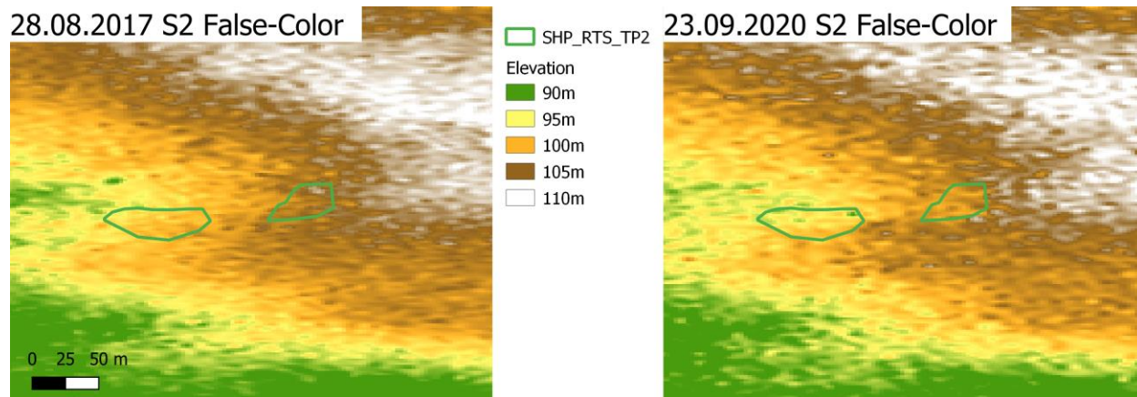
Figure 1: Left: DEM generated in winter 2017/18, Right: DEM generated in Winter 2010/21
