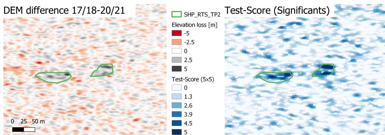
Figure 2: Left: DEM difference between winter 2017/18 and winter 2020/21, Right: Test (Significant) Score using a 5x5 moving window. This takes into account the the errors in the elevation measurements (see Bernhard et al. 2020 for a detailed explanation of the Test-Score).
