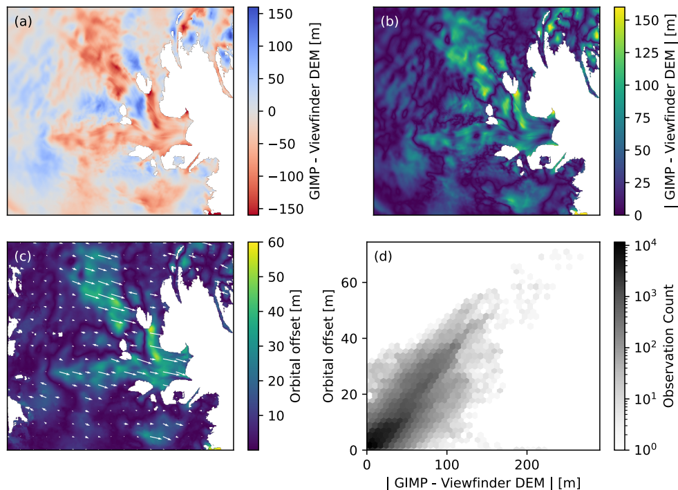
230 Figure 4: Comparison between DEM vertical differences and velocity offset for Helheim Glacier. (a) DEM difference between the Viewfinder DEM and the GIMP DEM. Areas where the GIMP DEM has a lower elevation value are in red, and a higher elevation value in blue. (b) Absolute vertical difference between the Viewfinder DEM and GIMP DEM. (c) Median offset between the measured displacement and expected displacement for velocity fields taken from relative orbits 053 and 139 (identical to fig. 3c). (d) Hexbin density plot comparing the absolute vertical differences between the Viewfinder DEM and GIMP DEM with the empirically determined orbital displacement.
