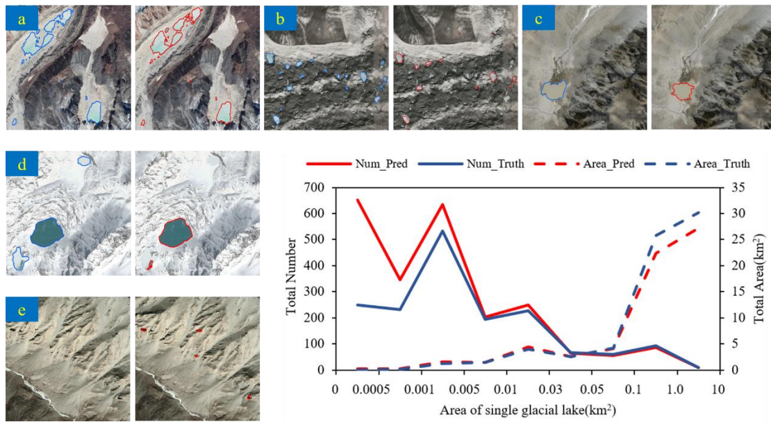
425 Figure 9. The display of glacial lake extraction results in different situations in the QNNR, as well as the statistics of area and number. All copyrights Image ©Google Earth 2020. The blue vectors are the boundary of the truth glacial lakes, and the red vectors are the boundary of the predicting results.
