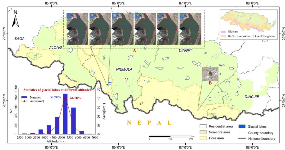
380 Figure 7. Glacial lake extraction result in the QNNR based on Google Earth images in 2020 (2.11 m). All copyrights Image ©Google Earth 2020.
