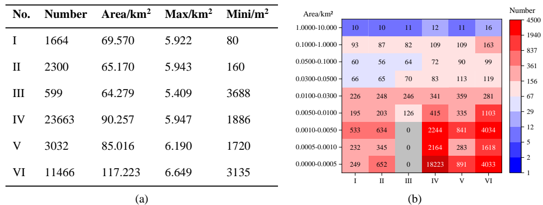
395 Figure 8. Comparison of glacial lakes between this study and the other four datasets.
