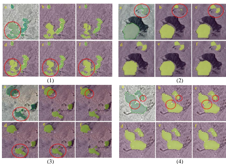
360 Figure 6. Comparison of glacial lake identification results based on Google Earth images (0.52 m) under different optimization conditions. All copyrights Image ©Google Earth 2020.
