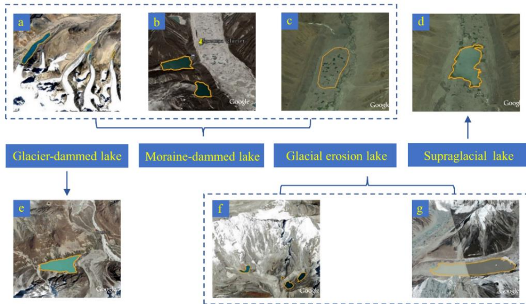
Figure 2. Seven types of glacial lakes in the training dataset. All copyrights Image ©Google Earth 2020.
