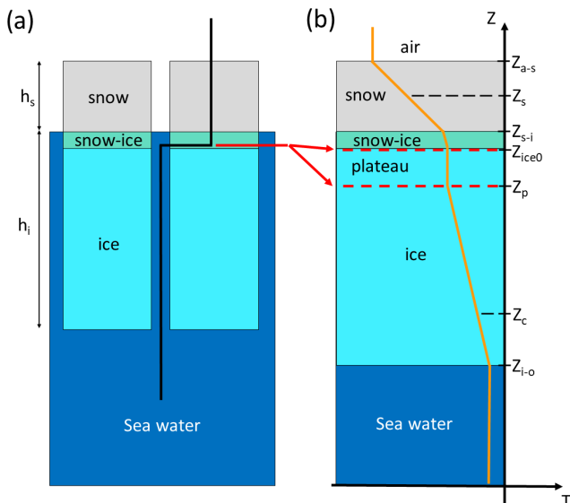
Figure 2. Schematics of the deployed SIMBA buoy thermistor strings through the snow, snow-ice and sea ice layers (a) and the vertical temperature profiles they measure, with the sensor positions identified by the surface retrieval algorithm (b). Note the section of the thermistor string (thermistor plateau, red lines) laid flat on the bare ice surface at deployment but later embedded within the ice layer after flooding. The marked sensor locations are, from top to bottom as follows: the air–snow interface ( Z_{a-s} ), the snow interior ( Z_s ), the snow–ice interface above the snow ice ( Z_{s-i} ), the snow–ice interface at deployment ( Z_{ice0} ), the lower end of the thermistor plateau ( Z_p ), a point in the ice interior close to the ice–ocean interface ( Z_c ) and the ice–ocean interface ( Z_{i-o} ).
