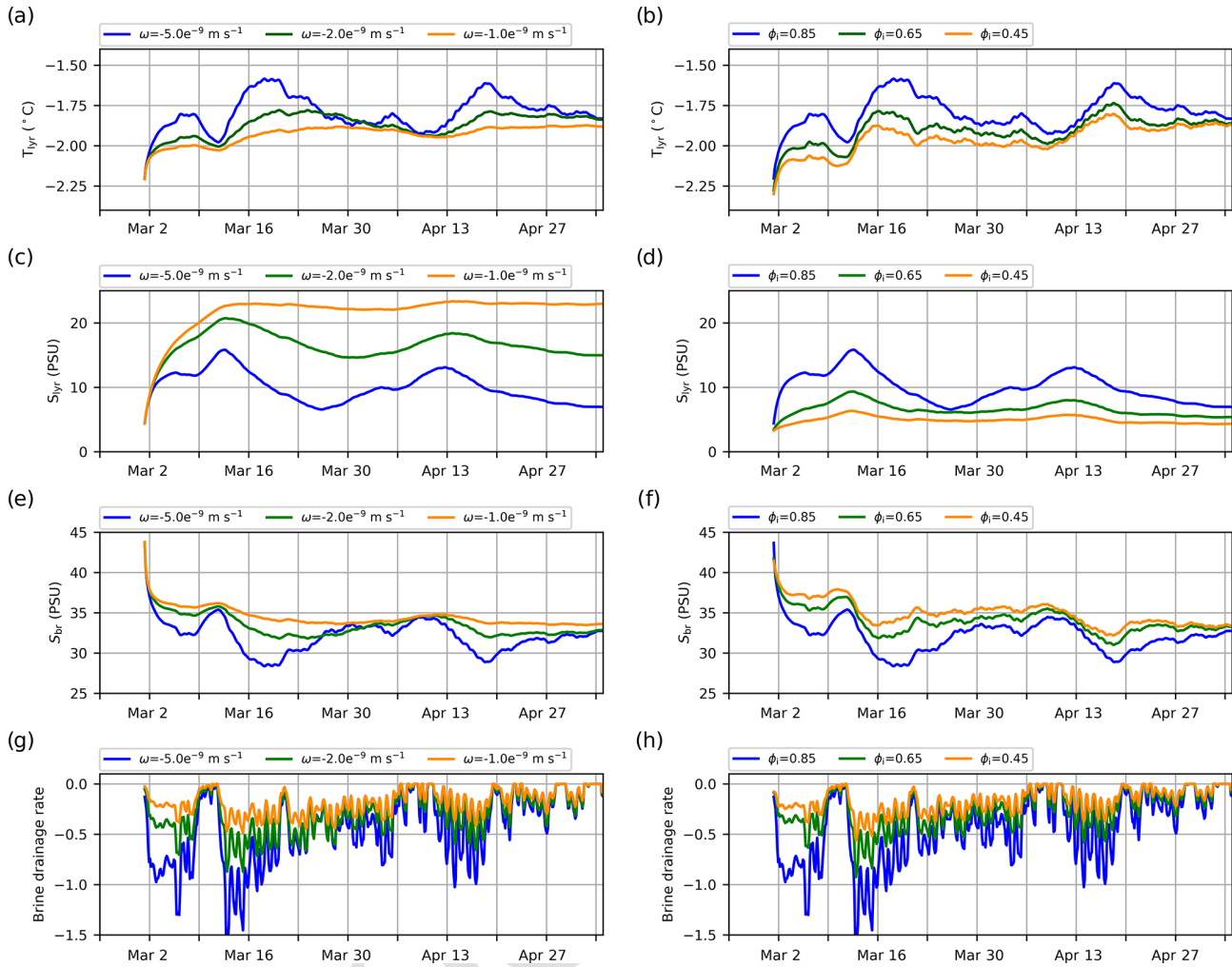
Figure 11. Time series of the temperature ( a , b ), bulk salinity ( c , d ), brine salinity ( e , f ) and brine desalination rate from the slow-brine-drainage parameterization ( g , h , represented in \text{psu d}^{-1} ), all in the lowest ice layer. Left panels show mushy-layer simulations using different brine drainage strength parameters \omega (using the standard congelation). Right panels show mushy-layer simulations using the different initial congelation liquid fraction \phi_{i\text{init}} and using the modified mushy-congelation scheme.
