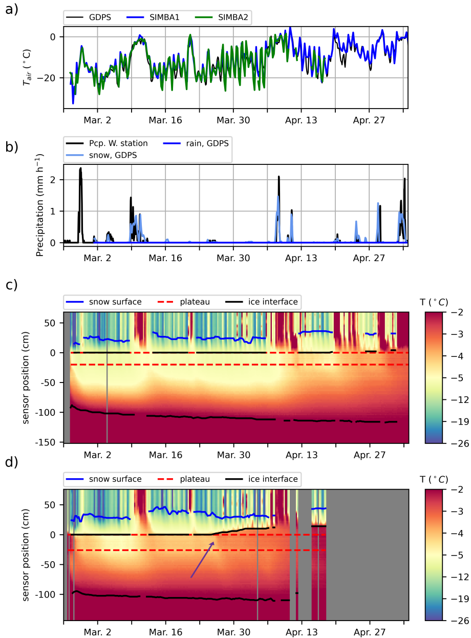
Figure 3. Time series of a) air temperature from the GDPS (black) and recorded by the IMB-SIMBA buoys ( IMB1-SIMBA1 in blue, IMB2-SIMBA2 in green); b) precipitations from the Nain ECCC weather station (black) and from the GDPS (blue); c) recorded temperatures along the IMB1-SIMBA1 thermistor string (color) with the detected material interfaces ( air-snow-air-snow interface in blue, ice surface and bottom interfaces in black and thermistor string plateau in red); d) Same as (c) but for the IMB2-SIMBA2 buoy. The purple arrow points to the warming at the snow/ice-snow-ice interface, indicating flooding.
