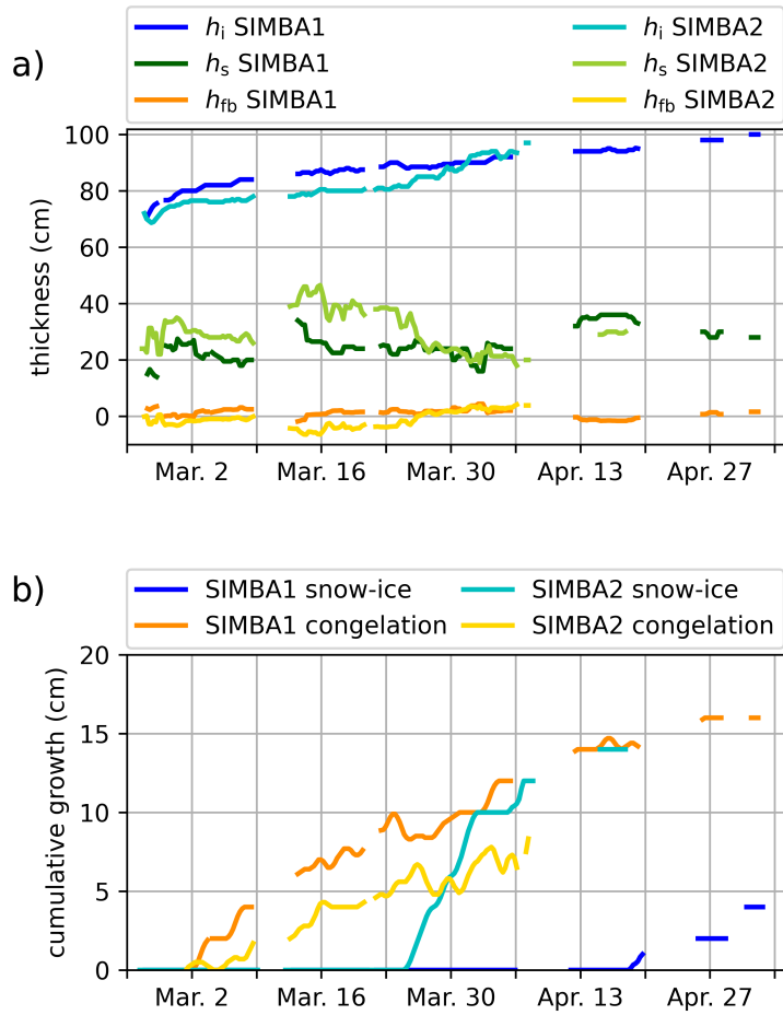
Figure 5. a) Ice (blue lines), snow (green lines), and freeboard (orange lines) thicknesses from the IMB-observationsSIMBA data . b) Contribution of snow-ice (blue lines) and congelation ice (orange lines) to the ice mass balance inferred from the IMB-observationsSIMBA data .
