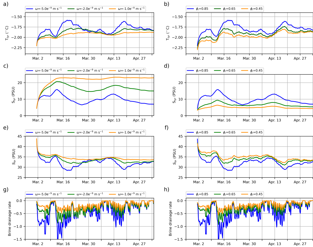
Figure 11. Time series of the temperature (a,b) temperature , bulk salinity (c,d) bulk salinity , brine salinity (e,f) brine salinity and desalination rate from the slow brine drainage parameterization (g,h, in \text{PSU day}^{-1} ), all desalination rate (g,h) from the slow brine drainage parameterization in the lowest ice layer. Left panels: in mushy simulations with using different brine drainage strength parameters \omega (and using the standard congelation, left column ) and Right panels: in mushy simulations using different initial congelation liquid fraction \phi_{init} ( \phi_{init} , using the modified mushy congelation, right column ) scheme.
