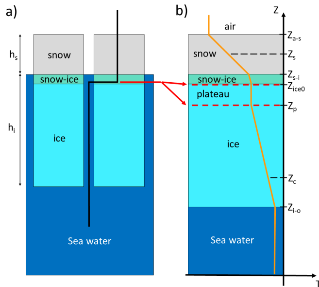
Figure 2. Schematics of the deployed SAMS-IMB-SIMBA buoy thermistor strings through the snow, snow-ice and sea ice layers (a) and the vertical temperature profiles they measure (b), with the sensor positions used in identified by the surface retrieval algorithm (b). Note the section of the thermistor string (thermistor plateau, red lines) laid flat on the bare ice surface at deployment but later embedded within the ice layer after flooding. The marked sensor locations are, from top to bottom: the air-snow interface ( Z_{a-s} ), the snow interior ( Z_s ), the snow-ice interface above the snow-ice ( Z_{s-i} ), the snow-ice interface at deployment ( Z_{ice0} ), the lower end of the thermistor plateau ( Z_p ), a point in the ice interior close to the ice bottom ( Z_c ), and the ice-ocean interface ( Z_{i-o} ).
