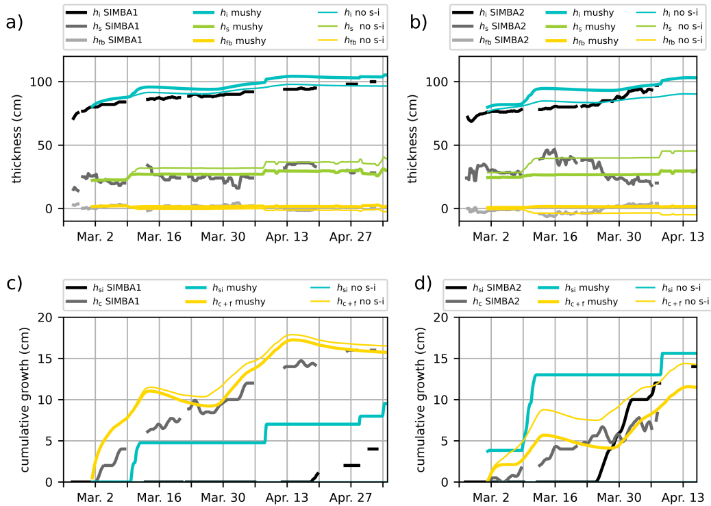
Figure 8. Ice mass balance in the mushy layer simulations against the IMB1-SIMBA1 (a,c) and IMB2-SIMBA2 (b,d) observations. Top pannels-panels (a,b): ice thickness (blue lines), now-snow depth (green lines) and freeboard (yellow lines) values, with the IMB -observations in black. Bottom pannels-panels (c,d): cumulative ice growth from ice bottom (yellow lines, including frazil ) and snow-ice formation (blue lines), with the IMB -observations in black. Thin lines indicate results from the mushy simulations ran without using the snow-ice parameterization.
