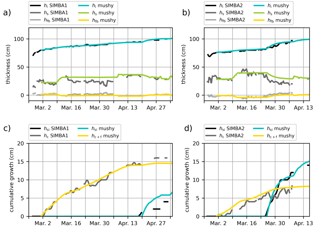
Figure 12. Ice mass balance in the-mushy layer simulations tuned to best represent the observations against from the IMB1-SIMBA1 (a,c) and IMB2-SIMBA2 (b,d) records-buoys (observations are in black). The snow flooding onset is set manually according to the observed flooding onset dates, and the simulations use the modified congelation scheme with \phi_{init} = 0.45 . Top panels (a,b): ice thickness (blue lines), snow depth (green lines) and freeboard (yellow lines) values, with the IMB observations in black. Bottom panels (c,d): cumulative ice growth from ice bottom (yellow lines, including frazil) and snow-ice formation (blue lines), with the IMB observations in black.
