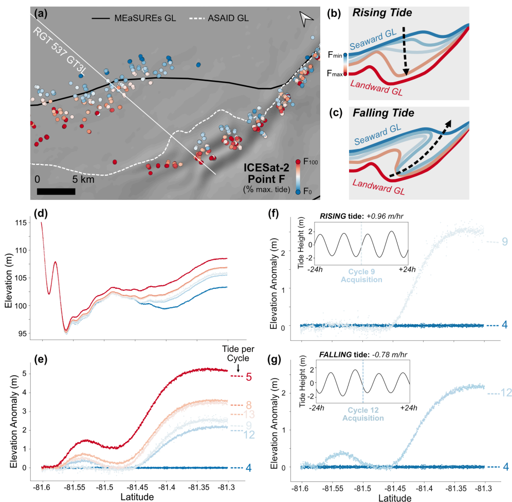
Figure 7: (a) The spatial pattern of tidal GL migration observed in Area B, Bungenstockrücken. Point F identified for every repeat cycle of each ICESat-2 ground track is coloured by % of maximum tide height. (b-c) Schematics depicting the flow of water in between the seaward and landward GL positions inferred from ICESat-2 RTLA results in Area B, during the rising and falling tide phase. (d-e) The repeat elevation profiles and anomalies of RGT 537 GT3L, calculated using the lowest-sampled tide reference profile from cycle 4. Repeat cycles are coloured by tide (as % of maximum tide height), and the cycle numbers are labelled in (e) alongside the CATS2008 modelled tide heights, differenced from the tide at cycle 4. (f-g) The individual elevation anomalies for cycles 9 and 12 against the lowest-sampled tide profile of cycle 4. Inset panels show the time-series of tide heights for the 24 hours before and after the time of ICESat-2 overpass at each cycle, showing the coincident tide phase and velocity .
