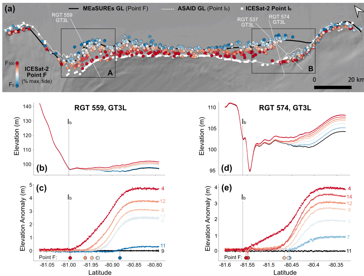
Figure 4: Tidal GL migration at Bungenstockrücken, measured by ICESat-2 RTLA. (a) The location of Point F at every sampled repeat cycle per ICESat-2 ground track is coloured by % of maximum tide height, overlain on the REMA 8m DEM (Howat et al., 2018), MEaSUREs GL (Rignot et al., 2016), ASAID break-in-slope GL (Bindschadler and Choi, 2011), and the most recent ICESat-2 derived break-in-slope (Point I b ) along each ground track (Li et al., 2022c). The two areas with the largest observed GL migration are highlighted as Areas A and B, and the locations for RGT 559 GT3L, 537 GT3L and 574 GT3L are shown. (b-c) The repeat elevation profiles and anomalies of RGT 559 GT3L, with repeat cycles coloured by tide (as % of maximum tide height) and labelled in (c). The location of ICESat-2 Point I b is marked with a vertical dashed line (Li et al., 2022b). (d-e) The equivalent repeat elevation profiles and anomalies for RGT 574 GT3L.
