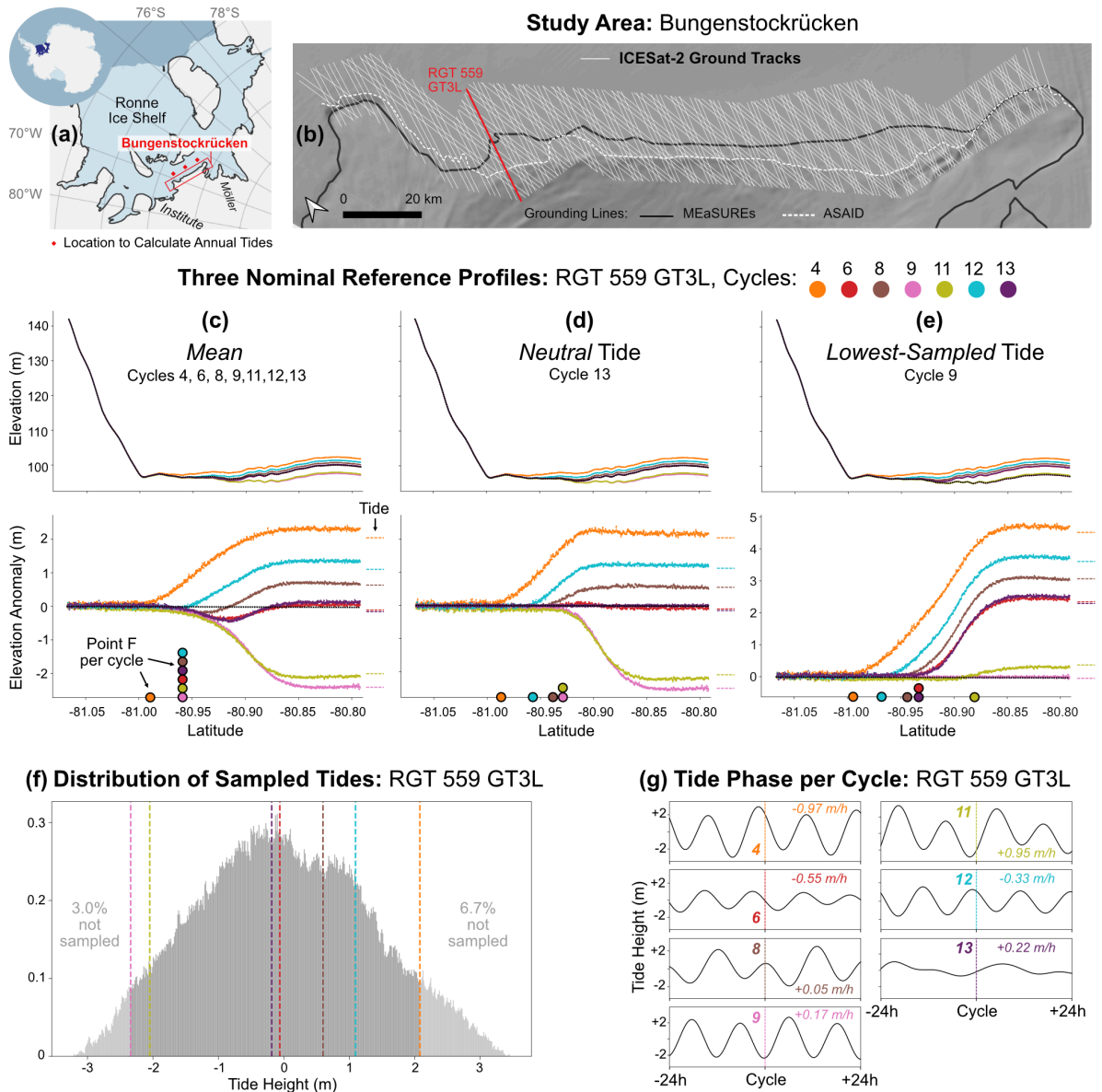
Figure 2: Method used to define three types of reference profile for elevation anomaly calculations along ICESat-2 ground tracks, as 180 illustrated for RGT 559 GT3L at the Bungenstockrücken ice plain. (a) Location of Bungenstockrücken on the Ronne Ice Shelf. Red diamonds show the locations used to calculate annual tide distributions. (b) ICESat-2 ground tracks crossing the MEaSURES and ASAID GLs in the study area (Rignot et al., 2016; Bindshadler and Choi, 2011). (c-e) Repeat surface elevation profiles and anomalies of RGT 185 559 GT3L, each using a different reference profile: (c) mean profile of cycles 4, 6, 8, 9, 11, 12, 13; (d) neutral profile of cycle 13; (e) lowest-sampled tide profile of cycle 9. The reference profile at zero-elevation anomaly is shown as a black dashed line, and the latitude of the derived Point F positions for each cycle along-track as coloured circles along the x-axis. Dashed coloured lines show the modelled tide height at the time of each cycle at the most seaward point along-track (in (e) these are differenced from the tide of cycle 9). (f) Histogram of CATS2008 modelled tide heights experienced over a single year, centred on 01/01/2020 (Howard et al., 2019), with vertical coloured dashed lines showing the tide height at each repeat cycle. (g) Tidal time series showing tide height, velocity and phase during the 24 hour period before and after the ICESat-2 overpass for each repeat cycle at RGT 559 GT3L.
