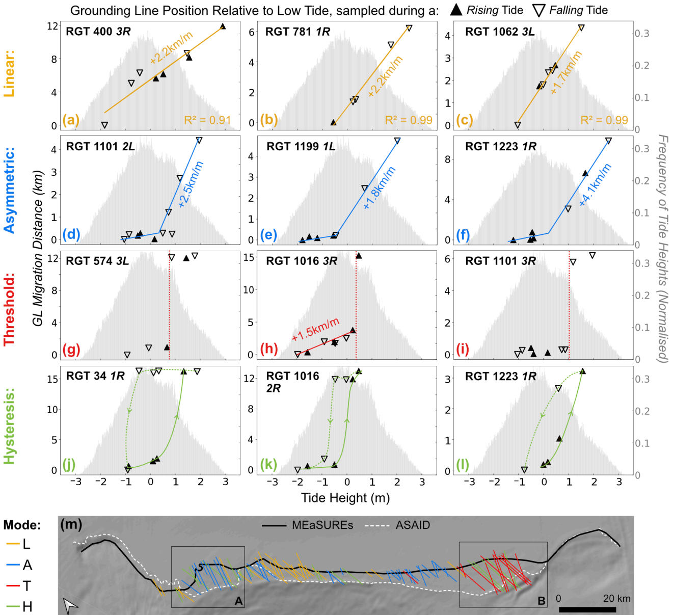
355 Figure 6: Four modes of tidal grounding line migration observed along ICESat-2 ground tracks at Bungenstockrücken. Three examples are shown per mode, which are classified from top to bottom as: (a-c) Linear, with a linear relationship between tide height and GL migration distance; (d-f) Asymmetric, with higher tides causing an increased rate of GL migration; (g-i) Threshold, with a sharp tide 360 threshold above which there is significant GL migration; (j-l) Hysteresis, with a difference in the impact of tidal variability on GL migration during the rising vs falling tide phase. In each example we show the along-track migration distance between each Point F and the Point F measured at the lowest-sampled tide as a function of coincident tide height from CATS2008 (Howard et al., 2019). Note the variable y axis scale between ground tracks. The orientation of the triangle indicates whether the repeat cycle was sampled during a rising or falling tide phase. Histograms show the distribution of tide heights experienced across a single year, centred on 01/01/2020. (m) Map of Bungenstockrücken showing ICESat-2 ground tracks coloured by migration mode (excluding tracks with <1 km tidal migration or <2 m tide range sampled).
