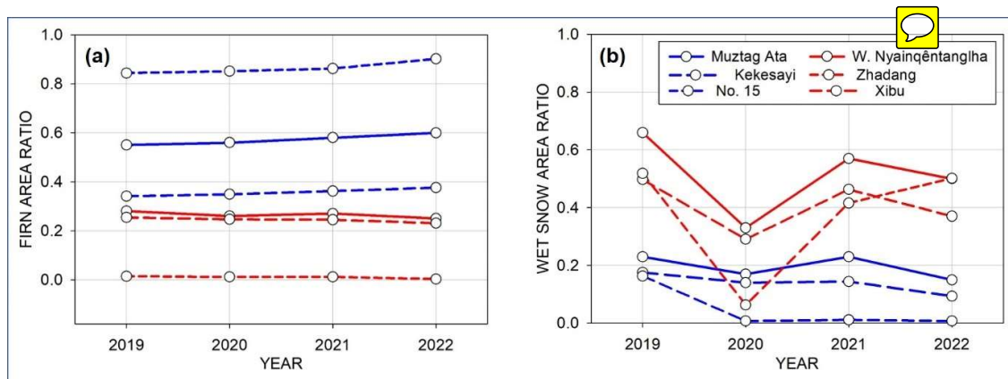
540 Figure 7. Evolution of the firn area– (a) and wet snow area–ratio (b) between 2019 and 2022.
