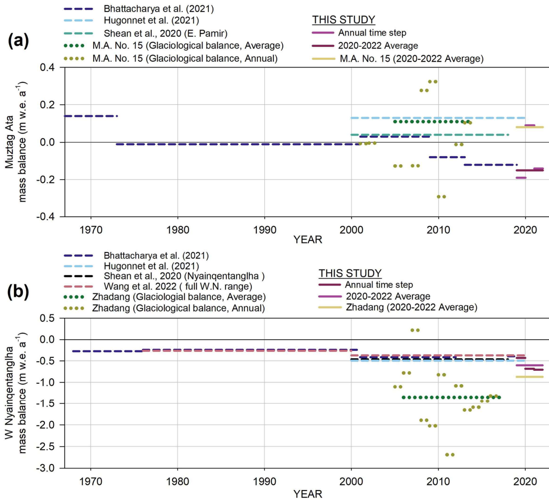
Figure 8. Comparison of geodetic glacier mass balance for the total glacier area and specific glaciers with available glaciological mass balance records in Muztag Ata (a) and Western Nyainqêntanglha (b).
