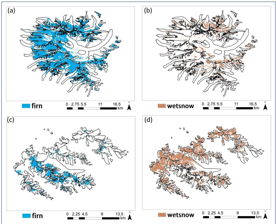
505 Figure 3. Examples of firn and wet snow cover retrieval in winter and summer 2021 in Muztag Ata (a, b) and Western Nyainqentanglha (c, d).
