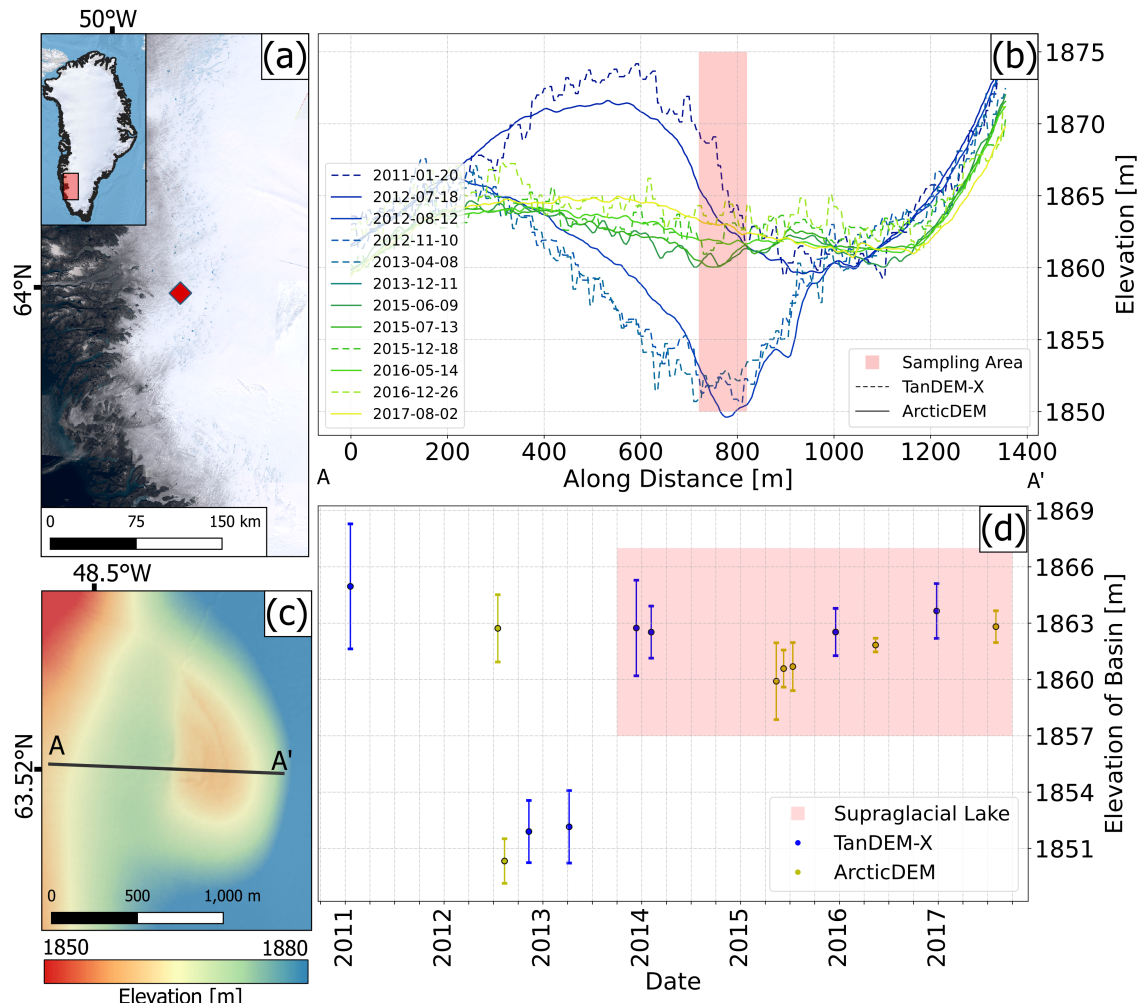
Figure 11. Possible active subglacial lake: (a) The location of the collapse basin on a background image from Landsat-8 from 2019. (b) Elevation profiles from the two aligned data sets, TanDEM-X is the dashed line and ArcticDEM is the solid line. (c) Possible collapse basin as seen in an ArcticDEM, 12th of August 2012. Line A-A' is the profile used in Figure (b). (d) Time series of the deepest point of the lake basin from TanDEM-X (blue) and ArcticDEM (yellow).
