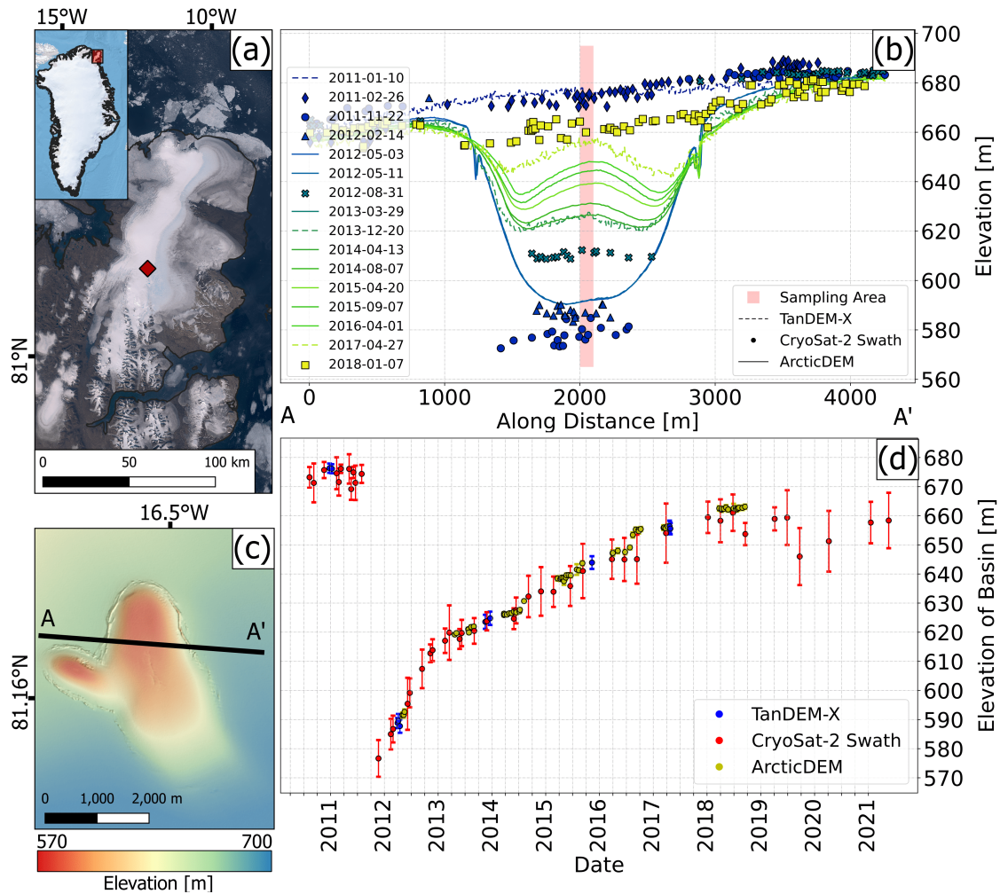
Figure 10. Lake 4 : (a) The location of the collapse basin on a background image from Landsat-8 from 2019. (b) Elevation profiles from the three aligned data sets; TanDEM-X is the dashed line, CryoSat-2 is represented by symbols and ArcticDEM is the solid line. c) The collapse basin as seen in an ArcticDEM, 3rd of May 2012. Line A-A' is the profile used in Figure (b). (d) Time series of the deepest point of the collapse basin from TanDEM-X (blue), CS2 (red) and ArcticDEM (yellow). The depth is based on sampling within the area indicated by red in (b)
