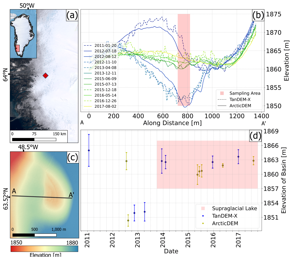
Figure 11. Possible active subglacial lake: (a) The location of the collapse basin on a background image from Landsat-8 from 2019 . (b) Elevation profiles from the two aligned data sets, TanDEM-X is the dashed line and ArcticDEM is the solid line. (c) Possible collapse basin as seen in an ArcticDEM, 12th of August 2012. Line A-A' is the profile used in Figure (b). (d) Time series of the deepest point of the lake basin from TanDEM-X (blue) and ArcticDEM (yellow).
