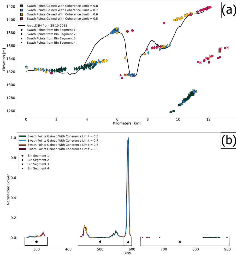
Figure 5. (a) Processed swath points from a CryoSat-2 11b Waveform (September 7, 2011) after the drainage event at Lake 1. The colours indicate what coherence limit was used to process each point and the symbols specify from where on the 11b waveform they are from. The dark green sections of the waveform are those accepted at a coherence threshold of 0.8, light blue sections are those additionally accepted from lowering the threshold to 0.7. Likewise, the yellow and pink are those for coherence thresholds of 0.6 and 0.5, respectively. The black line is the topography along the swath from an ArcticDEM scene from October 28, 2011. (b) Corresponding CryoSat-2 11b waveform, with the coloured sections illustrating what waveform part is gained when changing the coherence limit. The waveform is divided into four bin segments labelled by four distinctive symbols. The round points are from the early bin range at ~300, the diamond shapes are from the range at ~500, the triangles are from the large peak at ~600, and the crossed points are from the low power section after the large peak.
