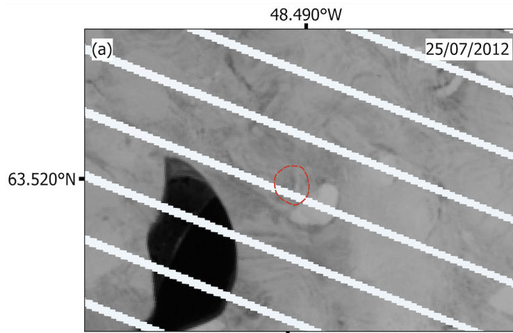
Figure A1. Landsat-7 images taken on July 25, 2012, over Lake 5 showing no signs of a collapse basin. The red outline indicated the collapse basin outline as created from an ArcticDEM from August 12, 2012.
