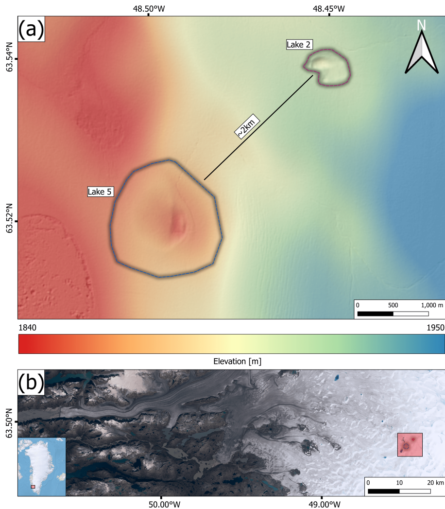
Figure A2. (a) Indication of the location of Lake 2 relative to Lake 5 shown on an ArcticDEM. (b) Overview of the two lakes' locations on a background image from Landsat-8 from 2019 .
