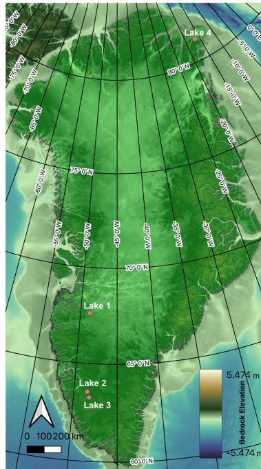
Figure 1. The locations of the four sites of active subglacial lakes investigated in this study shown on a background image of bedrock elevation from BedMachine v3 (Morlighem et al., 2017) .
