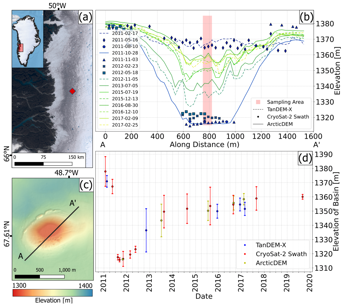
Figure 7. Lake 1 : (a) The location of the collapse basin on a background image from Landsat-8 from 2019. (b) Elevation profiles from the three aligned data sets; TanDEM-X is the dashed line, CryoSat-2 data is represented by symbols and ArcticDEM is the solid line. (c) The collapse basin as seen in an ArcticDEM, 28th of October 2011. Line A-A' is the profile used in Figure (b). (d) Time series of the deepest point of the lake basin from TanDEM-X (blue), CS2 (red) and ArcticDEM (yellow). The depth is based on sampling within the area indicated by red in (b)
