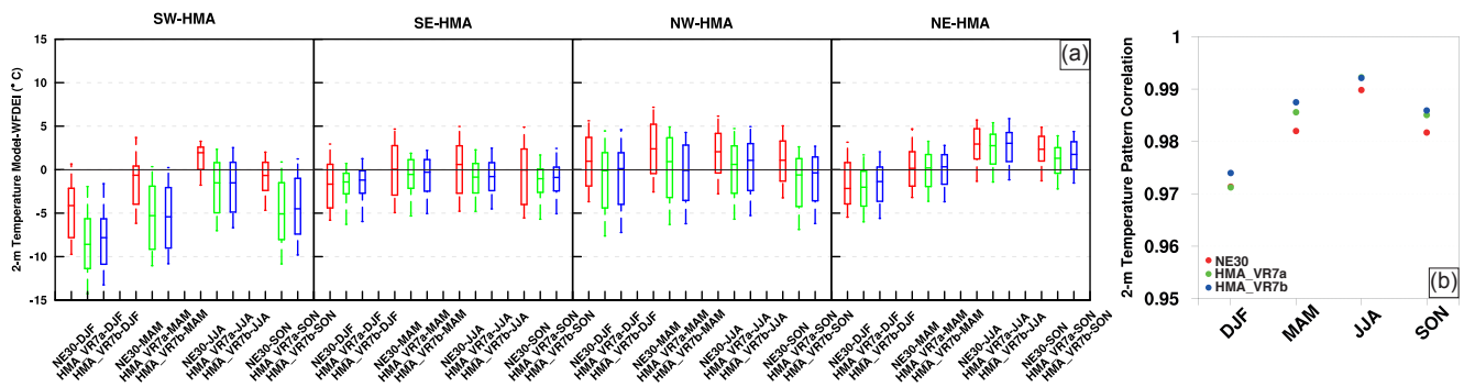
Figure 7. (a) Boxplots of 2-m temperature differences ( ^{\circ}\text{C} ) between the simulation outputs of NE30 (red), HMA_VR7a (green), HMA_VR7b (blue), and the observation/reanalysis-based WFDEI for each season and HMA subregion (shown in Figure 1b). The box represents the biases between the 25 th and 75 th percentile, the line in the box denotes the median, and the whiskers represent the 10 th and 90 th percentile of temperature differences. (b) Pattern correlations between the simulation outputs of NE30 (red), HMA_VR7a (green), HMA_VR7b (blue), and the observation/reanalysis-based WFDEI. The pattern correlations are calculated for each season and for the entire HMA region.
