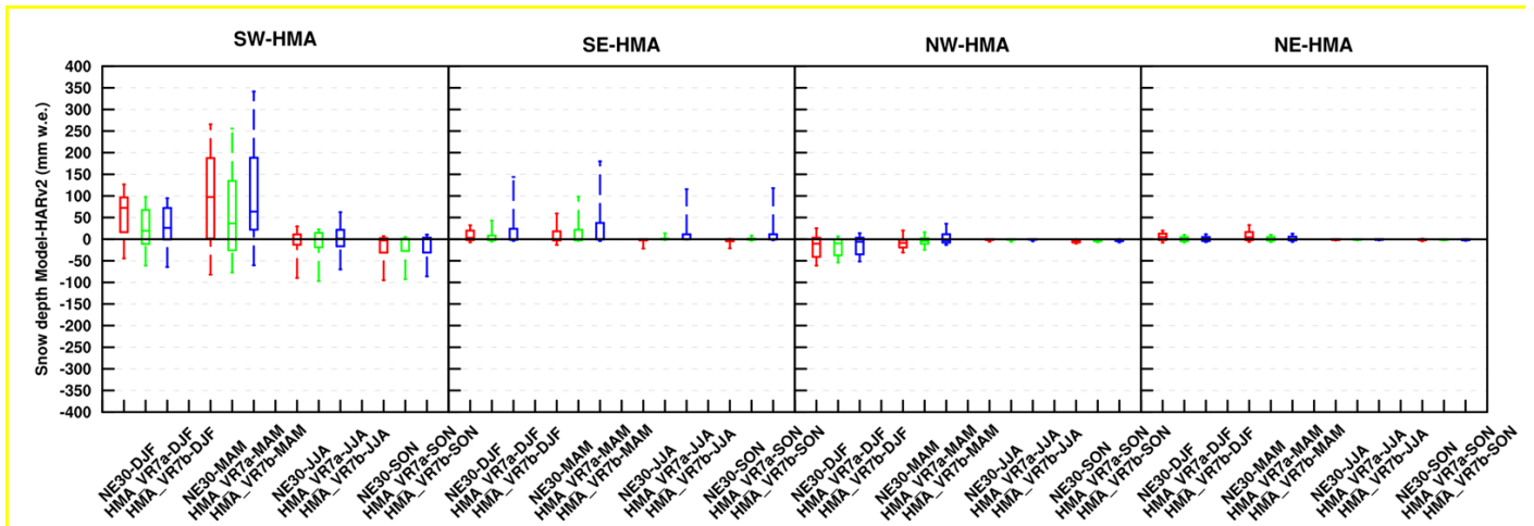
Figure RC2.1 Boxplots of snow depth differences (mm w.e.) between the simulation outputs of NE30 (red), HMA_VR7a (green), HMA_VR7b (blue), and HARv2 for each season and HMA subregion (shown in Figure 1b). The box represents the biases between the 25 th and 75 th percentile, the line in the box denotes the median, and the whiskers represent the 10 th and 90 th percentile of snow depth differences.
