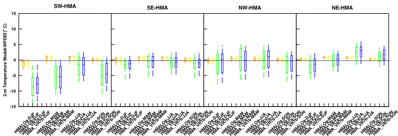
Figure RC1.1. Boxplots of 2-m temperature differences ( ^{\circ}\text{C} ) between the simulation outputs of HMALOa (orange), HMALOb (yellow), HMA_VR7a (green), HMA_VR7b (blue), and the observation/reanalysis-based WFDEI for each season and HMA subregion (shown in Figure 1b). The box represents the biases between the 25 th and 75 th percentile, the line in the box denotes the median, and the whiskers represent the 10 th and 90 th percentile of temperature differences.
